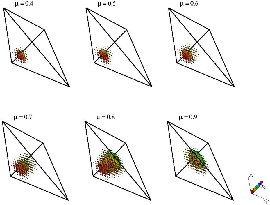
Figure 16. Population distribution \mathbf{p} for the JC mutation model with truncation selection (23) and x_c = 0.1 with a sequence length of N = 20 for varying mutation rates \mu .
