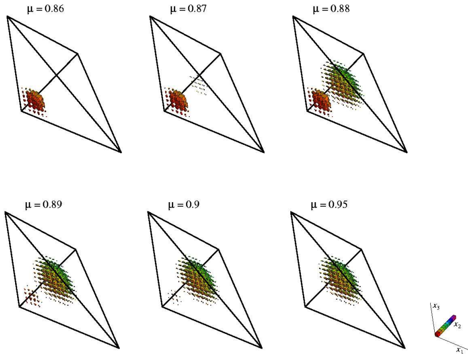
Figure 15. Ancestral distribution \mathbf{a} for the JC mutation model with truncation selection (23) and x_c = 0.1 with a sequence length of N = 20 for mutation rates \mu close to the error threshold.
