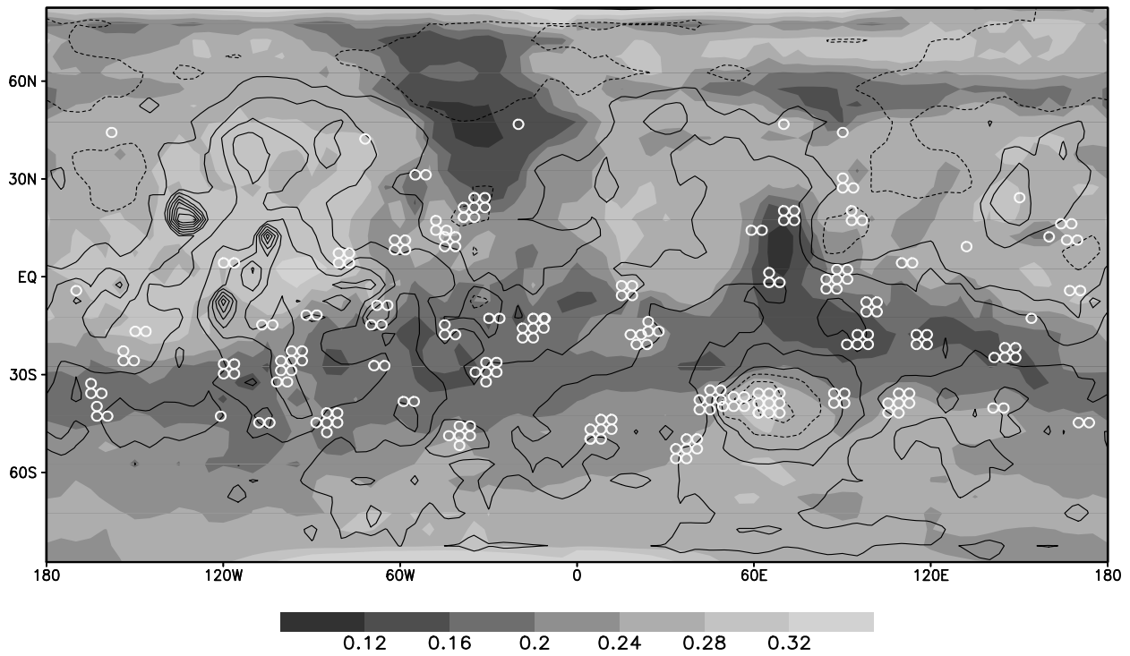
Figure 7: Approximate locations of early dust activity during onset of large Martian dust storms (data taken from a compilation by Martin and Zurek [1993] ). Also shown is height above the reference geoid (contours are every 2km and negative values are shown as dashed lines) and albedo (shading).
