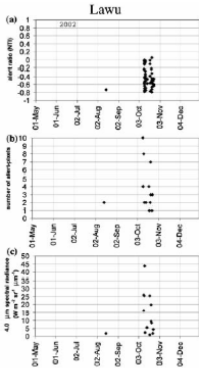
Figure 14 Time-series plots of MODVOLC thermal alerts for Lawu, which we believe to have been caused by fires. (a) alert ratio (NTI). (b) number of alert pixels on each overpass. (c) summed 4.0 \mu\text{m} radiance for alert-pixels.
