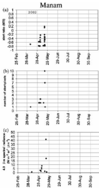
Figure 7 Time-series plots of MODVOLC thermal alerts for Manam. (a) alert ratio (NTI). (b) number of alert pixels on each overpass. (c) summed 4.0 \mu\text{m} radiance for alert-pixels. No MODVOLC thermal alerts occurred January 2001-March 2003 outside the time-period shown here.
