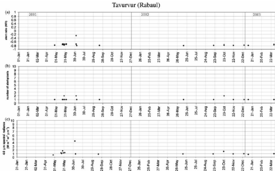
Figure 6 Time-series plots of MODVOLC thermal alerts for Rabaul (Tavurvur cone). (a) alert ratio (NTI). (b): number of alert pixels on each overpass. (c) summed 4.0 \mu\text{m} radiance for alert-pixels.
