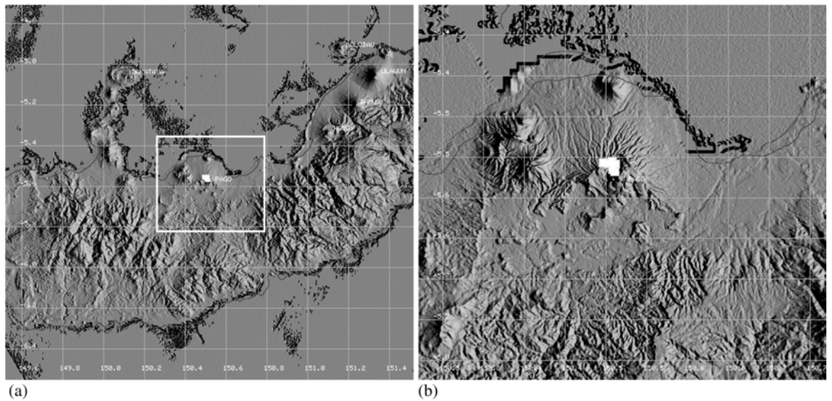
Figure 2 MODVOLC thermal alerts for 15 August 2002, taken from the MODIS Thermal Alerts website. (a) 2^\circ square centred on Pago (gridlines every 0.2^\circ , approx. 20 km), superimposed box identifies the area shown in (b), (b) 0.5^\circ square centred on Pago (gridlines every 0.05^\circ , approx. 5 km). Each consists of a topographic base with alert pixels superimposed. The alert pixels are the cluster of six overlapping white squares close to the centre of each view, and are displayed in colour on the website. In this example the alert pixels correspond to known intra-caldera lava effusion, which is discussed in the text. Exact centre co-ordinates of each alert pixel are provided in text files accessible at the website, which in this case also reveals that three of the alert pixels were detected by day and three by night.
