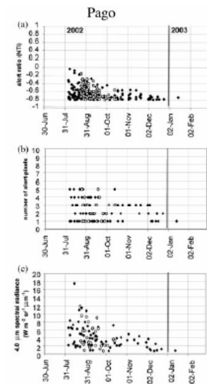
Figure 5 Time-series plots of MODIS thermal alerts for Pago. (a) alert ratio (NTI). (b) number of alert pixels on each overpass. (c) summed 4.0 \mu\text{m} radiance for alert-pixels. No MODVOLC thermal alerts occurred January 2001-March 2003 outside the time-period shown here. Two satellites provided MODVOLC data during this eruption: Terra (solid symbols) and Aqua (open symbols).
