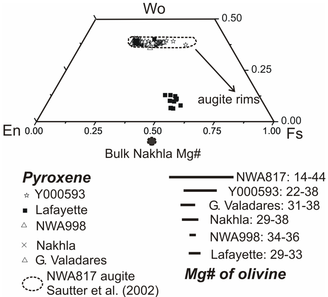
Fig. 4. Pyroxene and olivine compositions in the nakhlites. The main mineral phase in the nakhlites is an Fe-rich augite ( \text{En}_{0.37-0.62}\text{Wo}_{0.37-0.43}\text{Fs}_{0.24-0.41} ) with lesser amounts of pigeonite ( \text{En}_{48-54}\text{Wo}_{6-13}\text{Fs}_{35-39} ). There is little discernible compositional variation between 4 of the nakhlites (Nakhla, Lafayette, Governador Valadares, NWA998). However, Y000593 and NWA817 have the most Fe-rich augite core compositions – extending to \text{Fs}_{0.4} indicating that they have more fractionated assemblages. The arrow indicates the zonation of the augite rims to towards hedenbergite-like compositions, and this is most extreme in NWA817 augite. NWA817 also has the greatest range of olivine compositions ( \text{Fo}_{14-44} ) suggesting that it has undergone the least equilibration. Olivine grains compositions are plotted beneath the pyroxene quadrilateral. Their Mg# ratios are not in equilibrium with the pyroxene compositions or with the bulk Mg# of Nakhla (also plotted, 0.5) and this feature may be due to late crystallization of the olivine relative to the augite cores (e.g. see Fig. 9). The pyroxene and olivine compositions are from this study apart from the Y000593 olivine (Mikouchi et al. 2003) and the NWA817 augite, rims and olivine data (Sautter et al. 2002).
