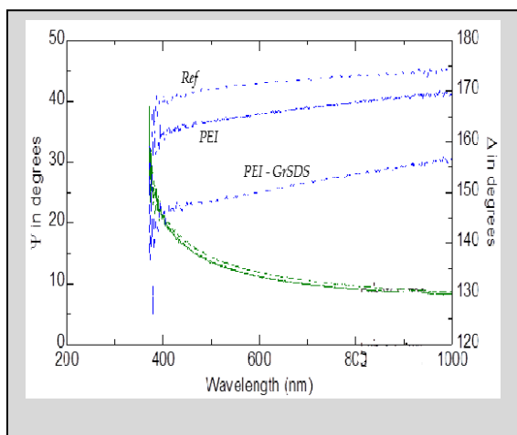
Fig. 3 Spectroscopic ellipsometry data for PEI/graphene-SDS layer on silicon.
