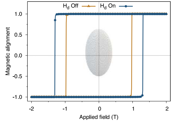
Figure 12. Simulated hysteresis loops for an ellipsoidal nanoparticle with an axial ratio of 2 showing the effect of the demagnetizing field calculated with the macrocell approach. A visualization of the simulated particle is inset.
