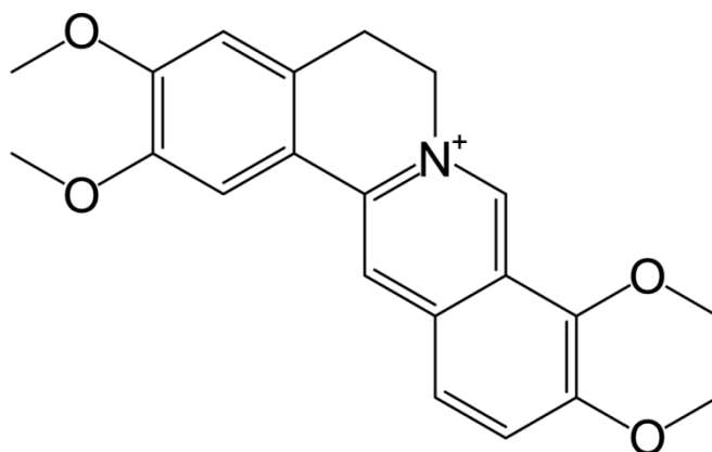
Fig.1. Chemical structure of Palmatine
