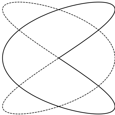
Fig. 2. The loops L_1 (black) and L_2 (dashed)
