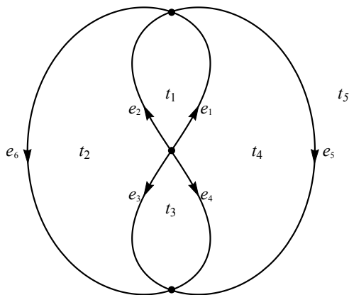
Fig. 3. A graph embedded in S^2 with five faces
