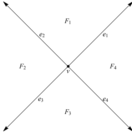
Fig. 5. The edges and faces at v
