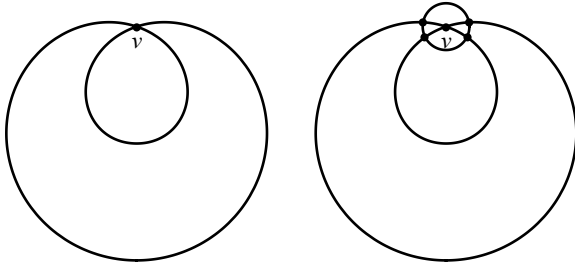
Fig. 6. A graph that is non-generic at v (left) and its generic counterpart
