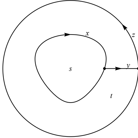
Fig. 4. The holonomy z around the boundary of the disk is constrained to lie in C .
