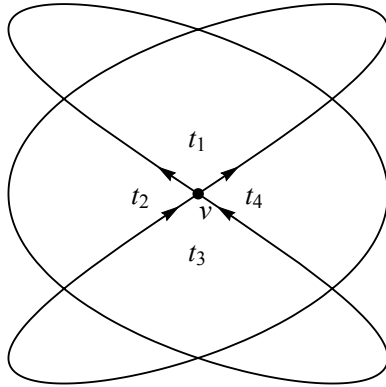
Fig. 1. A typical loop L for the Makeenko–Migdal equation
