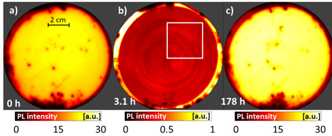
FIG. 7. PL images of a 1 \Omega\cdot\text{cm} p-type FZ sample from Group I featuring severe bulk lifetime degradation. The images are taken at 1 sun equivalent at different stages of LID indicated in the image. The sample was passivated with 10 nm P-ALD \text{Al}_2\text{O}_3 , capped by 100 nm PECVD a- \text{SiN}_x and fired at 900^\circ\text{C} . The dark rim in (a) and (c) and bright rim in (b) originate from the a- \text{SiN}_x capping layer not covering the whole wafer. Note that image (b) has a very different color scale and features distinct striations of 5%–10% _{\text{rel}} . The white square in (b) indicates the wafer section further investigated in Fig. 8.
