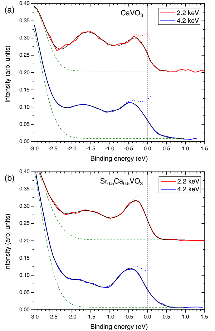
FIG. 3. (Color online) High-statistics HAXPES spectra of the V 3d states of (a) CaVO_3 and (b) Sr_{0.5}Ca_{0.5}VO_3 at 4.2 and 2.2 keV incident photon energies (vertically offset for clarity). The dashed (green) lines indicate the contributions from the tails of the O 2p band, and the black solid lines represent fits of the experimental spectra (see text). Finally, the dotted lines near E_F are the experimental spectra divided by the Fermi function (determined from Ag foil).
