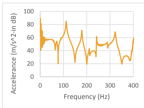
Fig. 2: Representative frequency response plot.
