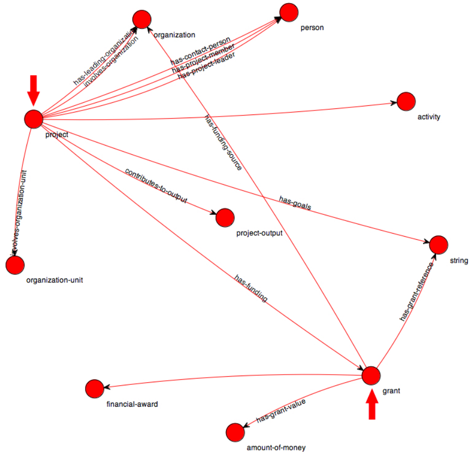
Fig. 2. Example of ontological-context for the \langle \textit{Project}, \textit{has} - \textit{funding}, \textit{grant} \rangle Statement.
