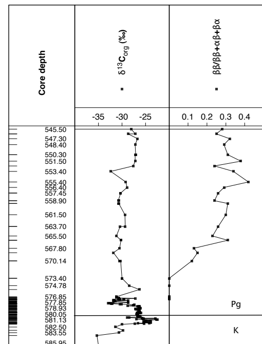
Figure 1 Carbon isotope stratigraphy for total organic matter and variations in the \text{C}_n \beta\beta/(\beta\beta+\alpha\beta+\beta\alpha) hopanoid maturity parameter in lowermost crater fill sediments from the Boltysch impact crater, Ukraine.
