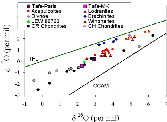
Figure 1: Oxygen Isotope Plot of Primitive Achond.
