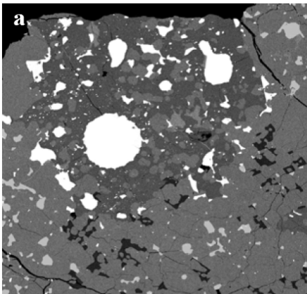
Figure 2: Figure 2a from [1] showing a relict chondrule similar to the chondrules in Renazzo
