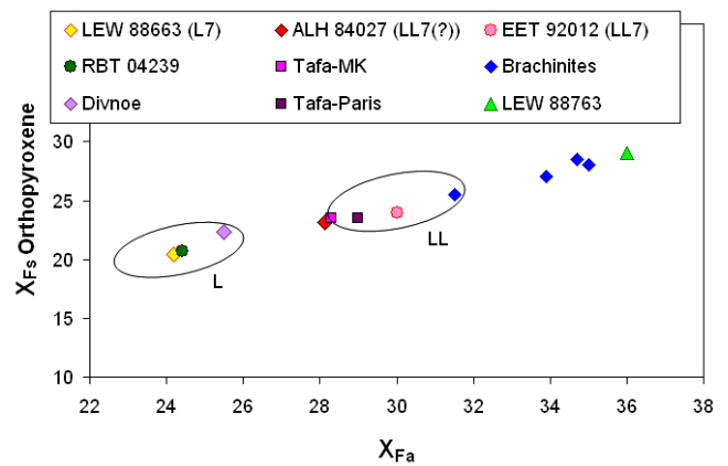
Figure 5: X_{\text{Fs,opxn}} vs. X_{\text{Fa}} for Primitive Achondrites and L and LL OCs
