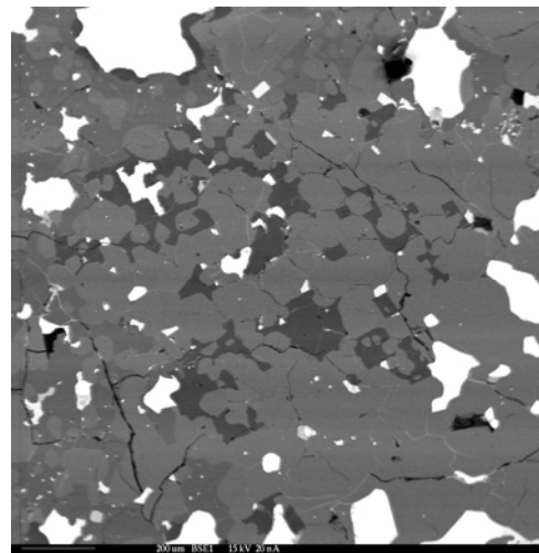
Figure 4: BSE image of Tafa-Paris (1.46 mm across)
