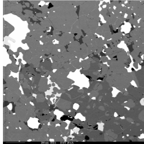
Figure 3: BSE image of Tafa-MK (1.46 mm across)
