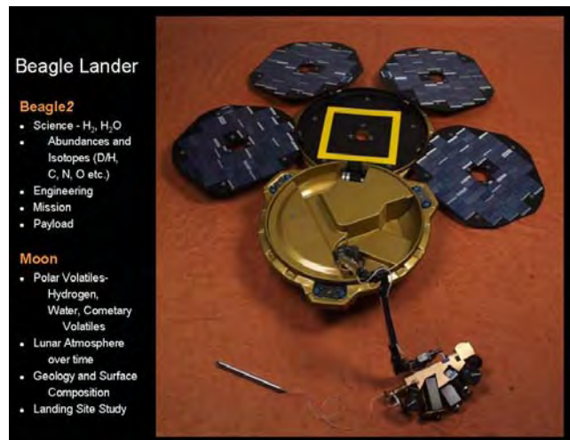
Figure 1. Beagle Lander Deployed
