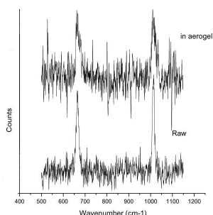
Figure 1. The Dispersive raman spectra for a pristine pyroxene grain and a grain captured in aerogel.
