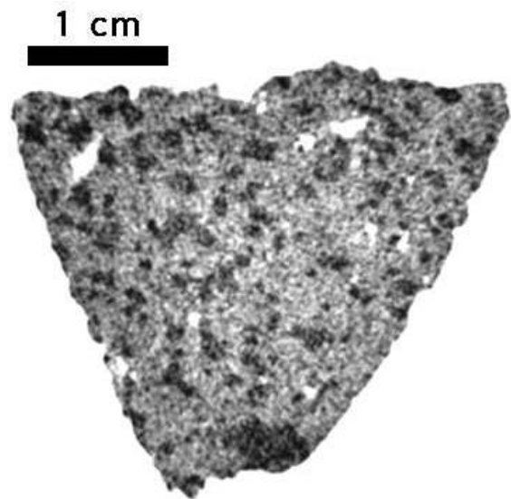
Fig. 1. Typical high-resolution X-ray tomogram of Sayh al Uhaymir 094 showing olivine crystals (dark) in groundmass and vesicles (bright).
