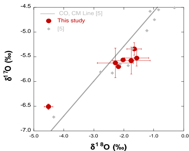
Figure 1 – Oxygen isotopic composition of CO3s. Only ALH77307 has an isotopic composition distinct from the rest of the CO3 meteorites. Error bars are 1\sigma on mean of replicates. Previous results [5] are shown for reference, as is the slope 0.70 line defined by bulk CO, CM and CM matrix samples [5].
