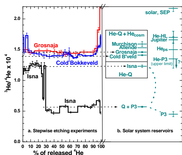
Fig. 1. ^3\text{He}/^4\text{He} release patterns during CSSE and ^3\text{He}/^4\text{He} ratios from different solar system reservoirs.
