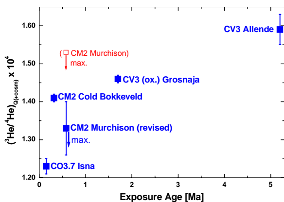
Fig. 2. ({}^3\text{He}/{}^4\text{He})_{\text{Q}+(\text{cosm})} vs. exposure age [26,27].
