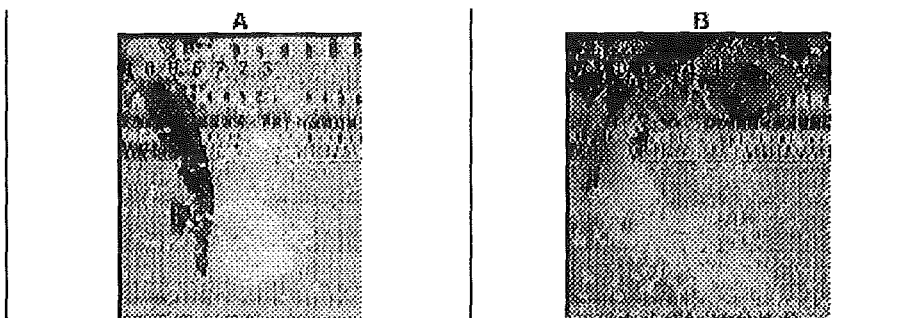
Figure 13 - Vortices generated during underwater undulatory motion.
