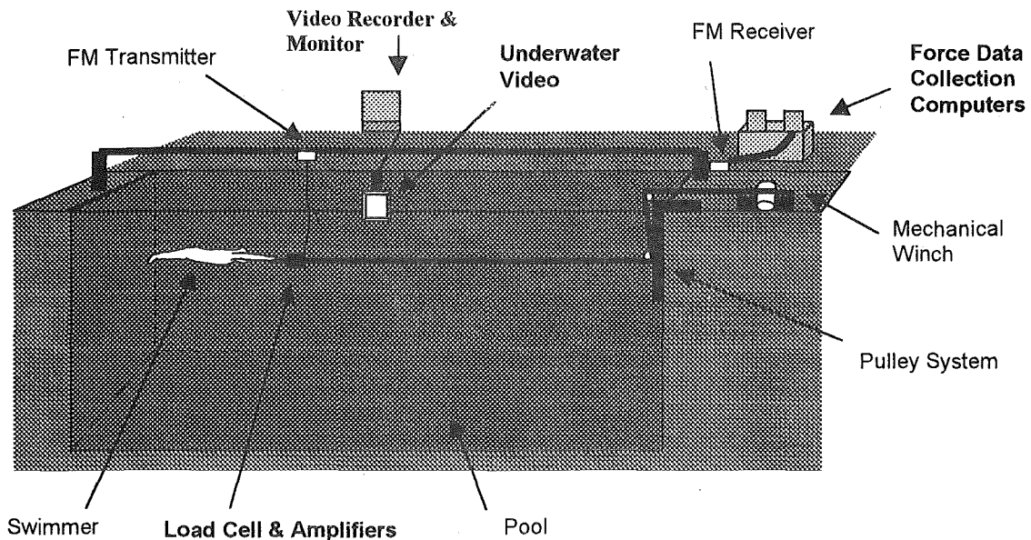
Figure 3 - Testing set-up for quantifying hydrodynamic drag.
