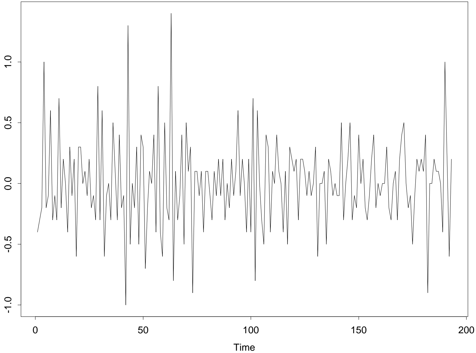
Time Series Plot of Diff. Series A
