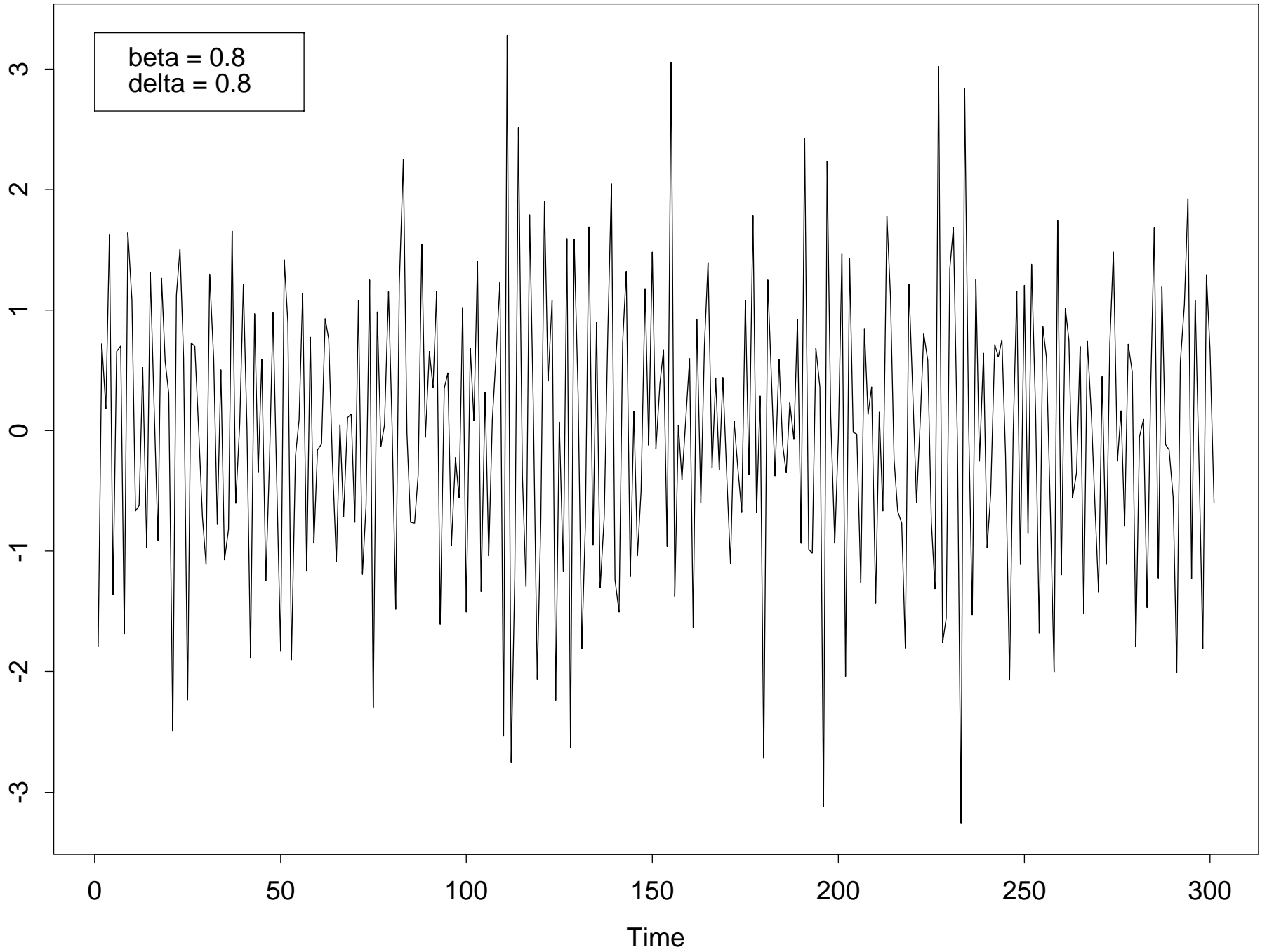
Time Series Plot of a GEMA(1)
