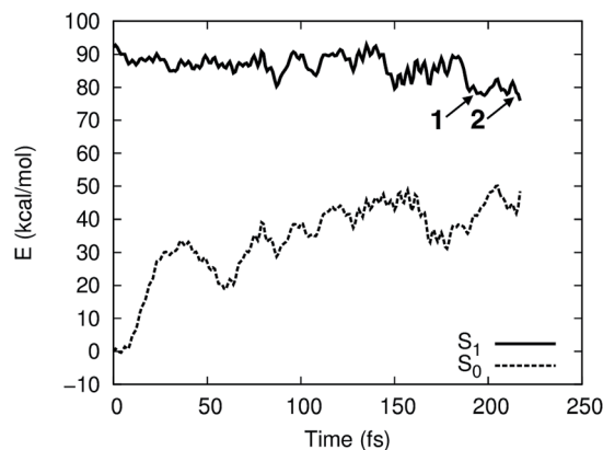
Fig. 2 Schematic presentation of the observed EPT reaction (a) and the S 1 and S 0 PESs for the reactive trajectory for (TiO 2 ) 4 (OH) 4 (H 2 O) 8 (b). In (a), blue and green colors indicate the location of the electron and the hole, respectively.
