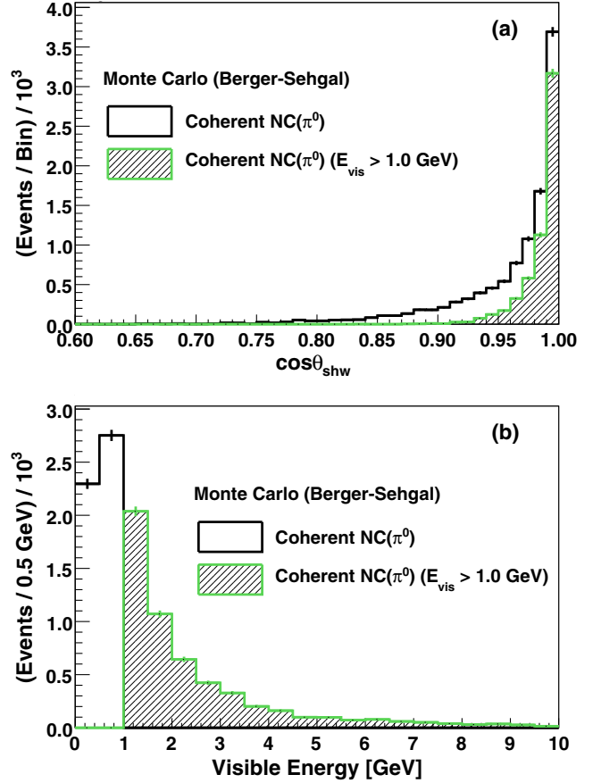
FIG. 3. Monte Carlo distributions for NC( \pi^0 ) coherent interactions (Berger-Sehgal model) in the Near Detector for the LE beam exposure. (a) Shower-angle cosine of final-state showers with respect to the \nu beam, and (b) event visible energies. Shaded regions show events with E_{\text{vis}} > 1 GeV.
