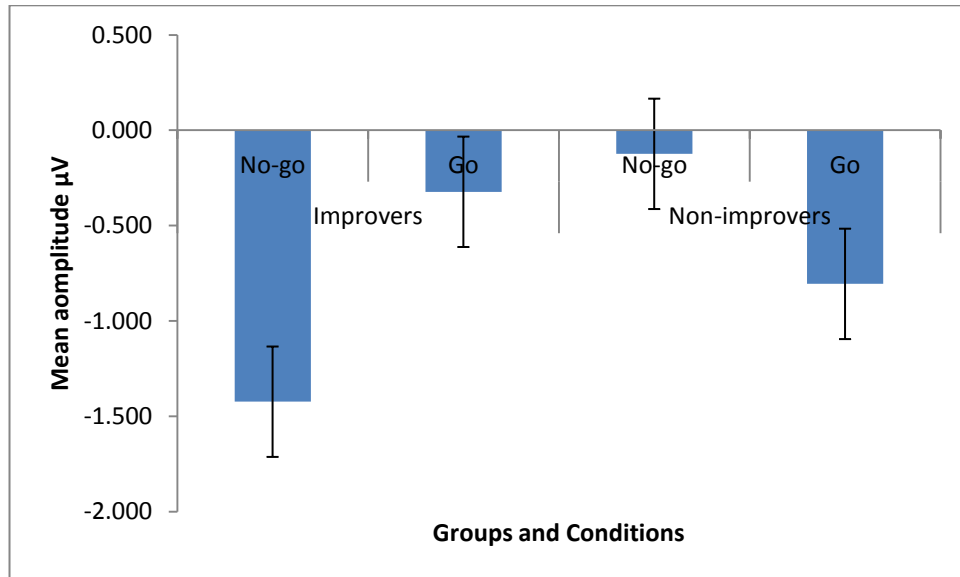
Figure 7: Mean (SE) N2 amplitudes in go and no-go trials for improver and non-improver male participants.
