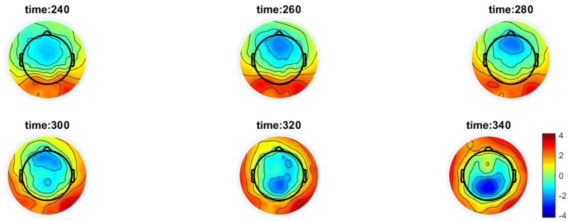
Figure 1a: Scalp maps showing N2 peak amplitude (dark blue) at about 260ms in frontal area, in a window of 240 to 340ms.
