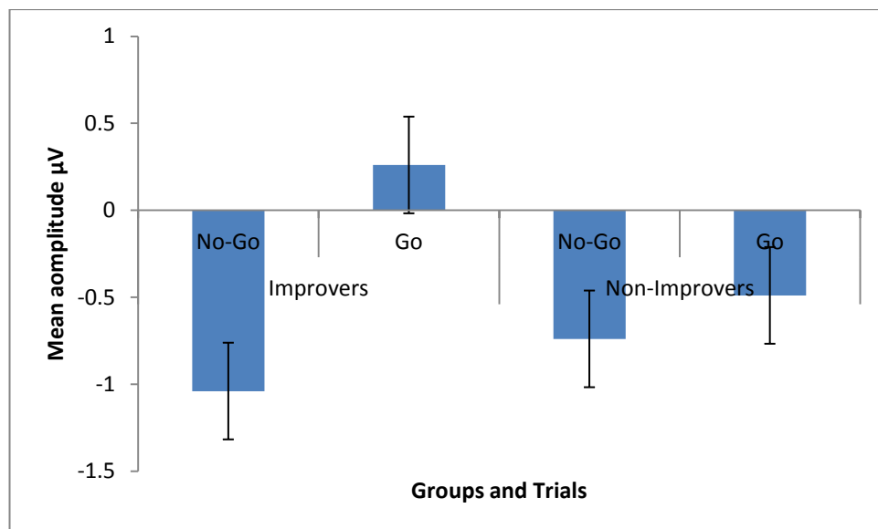
Figure 6: Mean (SE) N2 amplitudes for improvers and non-improvers for go and no-go trials.
