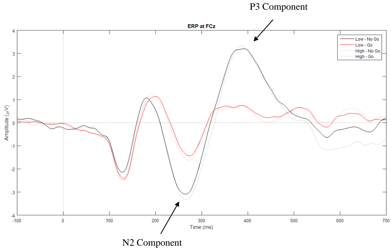
Figure 2: Grand Average ERPs for frontal N2 and P3 for high and low provocation and go and no-go trials
