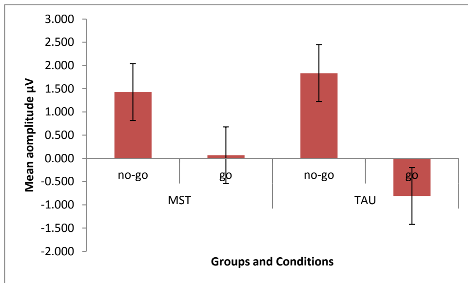
Figure 5: Mean (SE) P3 amplitudes in go and no-go trials for males in MST and TAU treatment groups.
