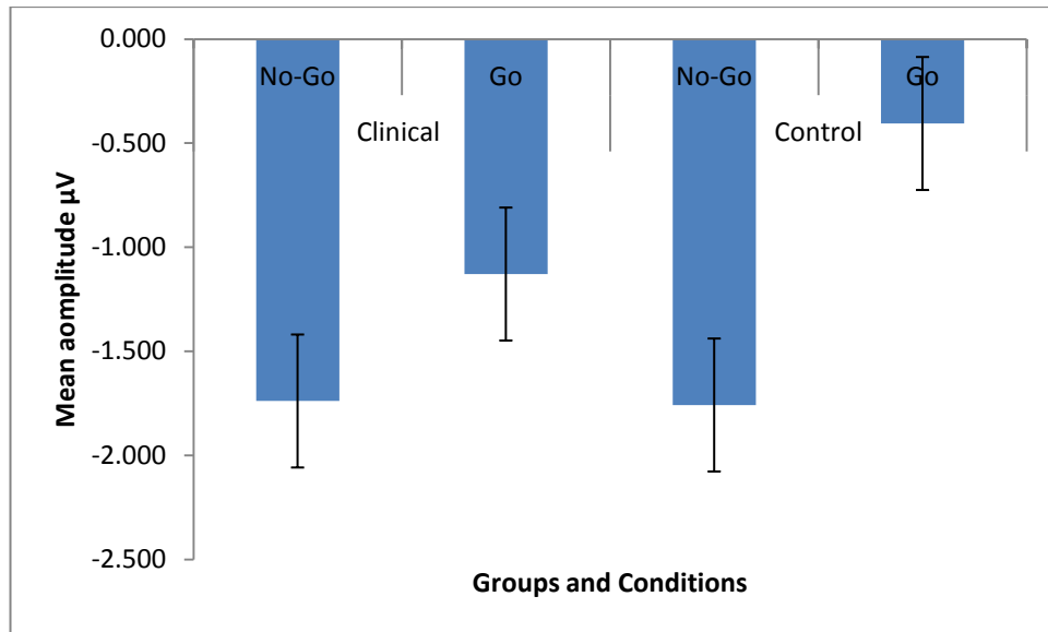
Figure 3: Mean (SE) N2 amplitudes in go and no-go trials for clinical and control male participants.
