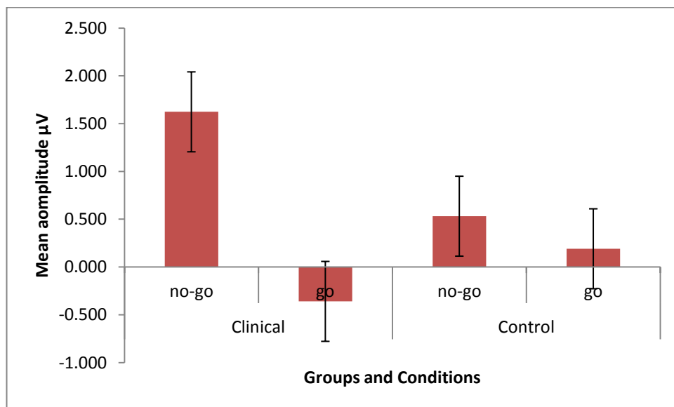
Figure 4: Mean (SE) P3 amplitudes in go and no-go trials for clinical and control male participants.
