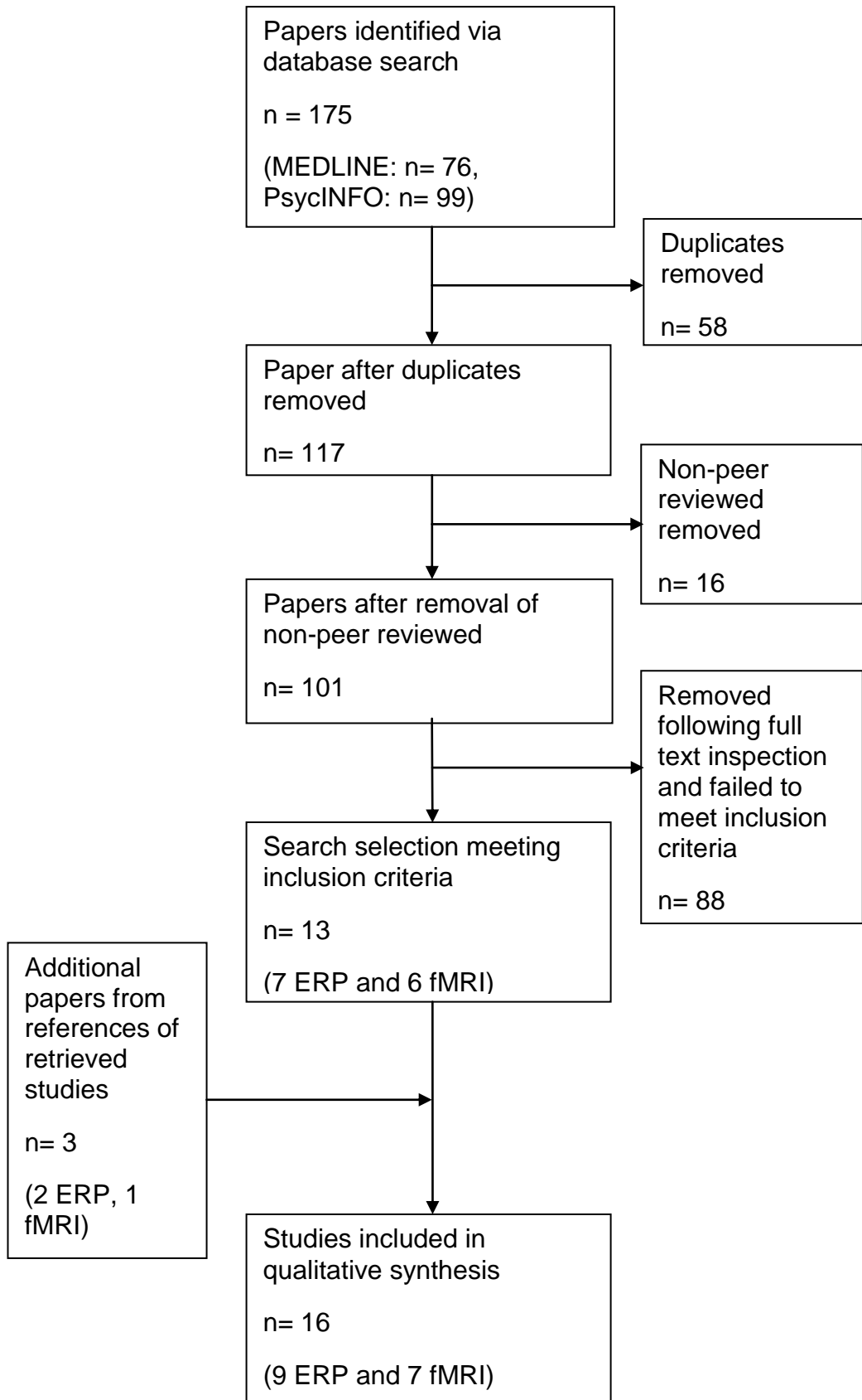
Figure 1: Paper selection and screening process
