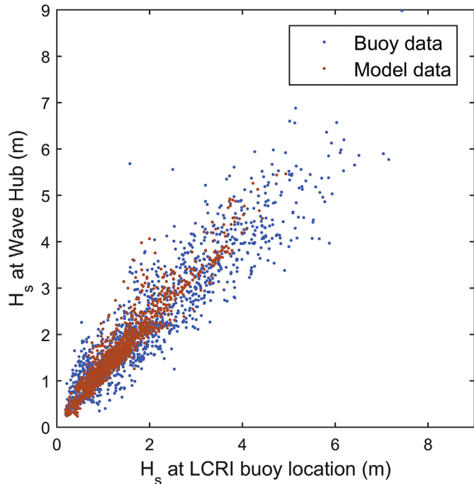
Fig. 7. Scatter plots of H_s at the WaveHub site against H_s at the LCRI site for both model and buoy data.
