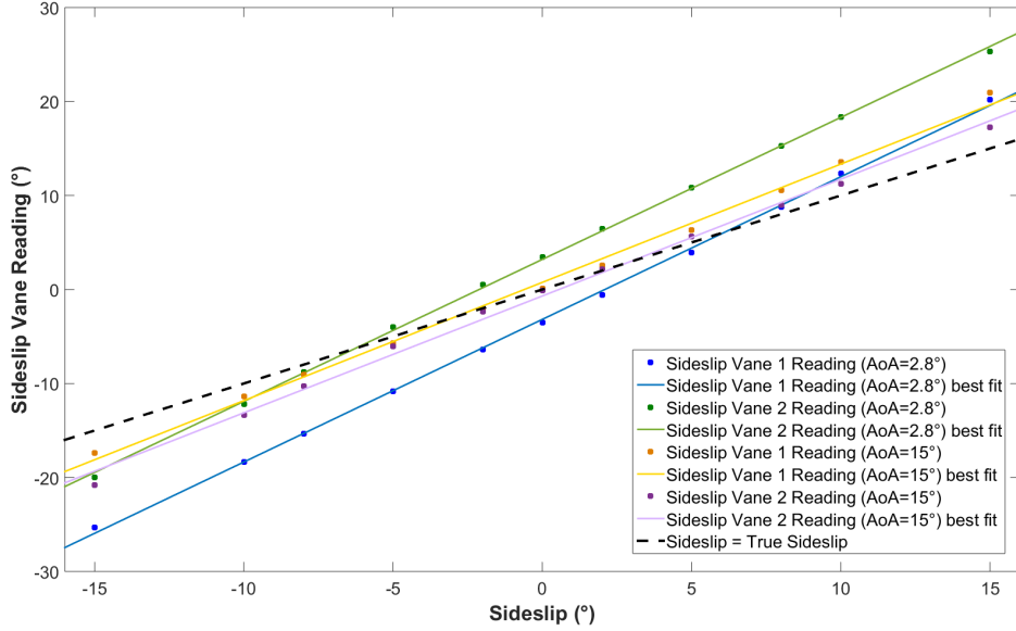
Figure 12: Difference in two sideslip vane readings for the cases AoA=2.8^\circ and AoA=15^\circ . Sideslip vane 1 is on the leading side of the nose for sideslip angles >0 , and sideslip vane 2 is on the leading side of the nose for sideslip angles <0 .
