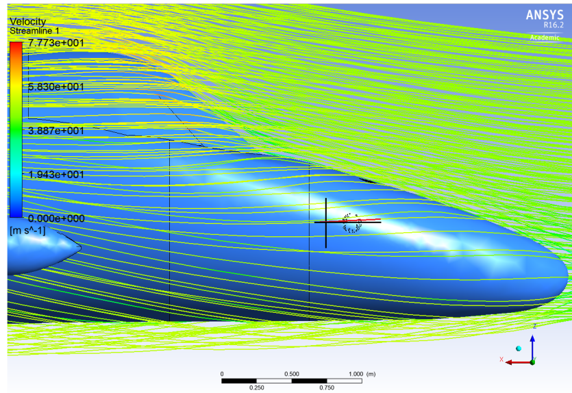
Figure 8: Effect of the nose on the local air flow direction around the angle of attack vane in the cases \alpha = 2.8^\circ, \beta = 15^\circ upper and \alpha = 2.8^\circ, \beta = -15^\circ right.
