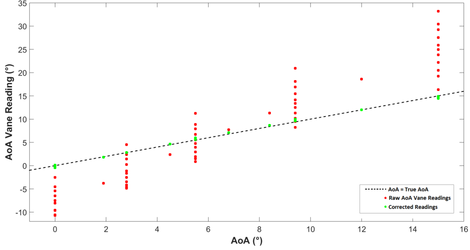
Figure 13: Equation (1) applied to the raw angle of attack vane data.
