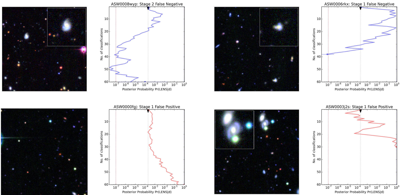
Figure 12. Illustrative examples of false negatives (blue) and false positives (red) from the classification of the SPACE WARPS –CFHTLS training set. The trajectory plot for each of the four subjects is shown to the right of its image. Left-hand panels show the most common types of trajectories: random walks with short steps resulting from no high-skill classifiers viewing the subject. The right-hand panels show examples where higher skill classifiers have been involved, causing larger, more efficient ‘kicks’ (top) but also catastrophic misclassifications (bottom right). Note that both these subjects were very nearly detected but did not quite reach the threshold set (marked by the blue dashed line). Insets for the false negatives show the lens feature. The inset for the lower right-hand panel shows where most volunteers believed a lens was located. There is no corresponding inset for the lower left-hand panel because no particular feature stood out to the citizens. Instead, the volunteers clicked many different features.
