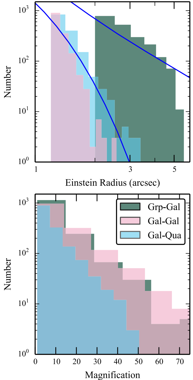
Figure 2. Einstein radius and total magnification distributions for all types of lenses. The solid (blue) curves show the theoretical prediction assuming an SIS model at galaxy scales and a total (NFW+Hernquist) model at group scales taken from More et al. (2012).
