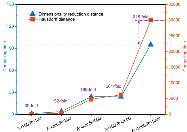
Fig. 7. Computing speed comparison between the two algorithms (different distance) at different feature points.
