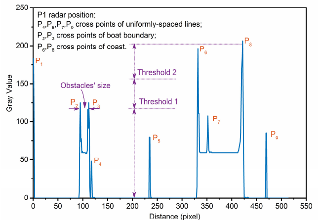
Fig. 3. Gray values of pixels of the auxiliary line in \alpha direction.
