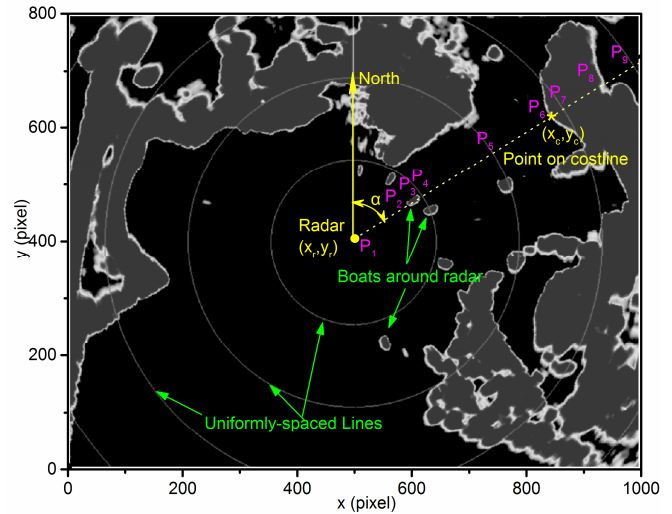
Fig. 2. Coastline extraction based on a radar image.
