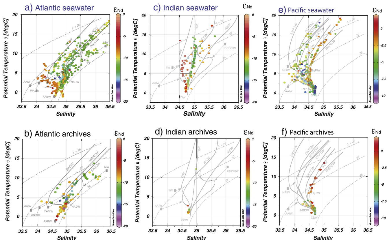
Fig. 6. Atlantic, Indian and Pacific T-S- \epsilon_{Nd} diagrams for seawater (a, c, e) and archives (b, d, f) at water depths from 200 m to bottom. Mean seawater \epsilon_{Nd} values of major water masses are summarized in Table 1, and the temperature and salinity ranges and the geographical extension of the water masses are shown in Table S2 (Emery and Meincke, 1986; Amakawa et al., 2009; Bostock et al., 2013). The figures and the maps are created using ODV (Schlitzer, 2015). Atlantic, Indian and Pacific T-S- \epsilon_{Nd} diagrams for seawater (a, c, e) and archives (b, d, f) at water depths from 200 m to bottom. Mean seawater \epsilon_{Nd} values of major water masses are summarized in Table 1, and the temperature and salinity ranges and the geographical extension of the water masses are shown in Table S2 (Emery and Meincke, 1986; Amakawa et al., 2009; Bostock et al., 2013). The figures and the maps are created using ODV (Schlitzer, 2015).
