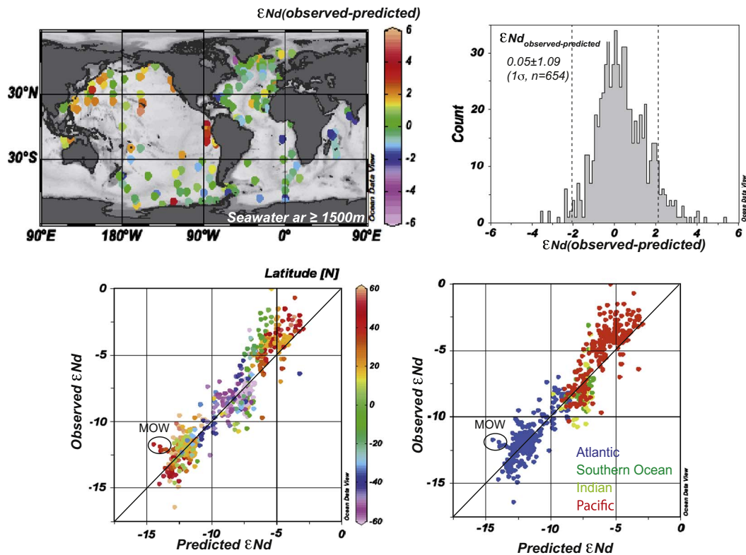
Fig. 8. Comparison between the predicted and observed global seawater \epsilon_{Nd} values. Map showing the distribution of difference between observed and predicted \epsilon_{Nd} values that correspond to -(\text{residual } \epsilon_{Nd}) values at \geq 1500 m (upper left panel). Histogram of -(\text{residual } \epsilon_{Nd}) values with 2\sigma interval (dashed lines, upper right panel). Scatter plots showing the correlation between observed and predicted \epsilon_{Nd} values with latitude (lower left panel) or with oceanic basins (lower right panel). The figures and the map are created using ODV (Schlitzer, 2015).
