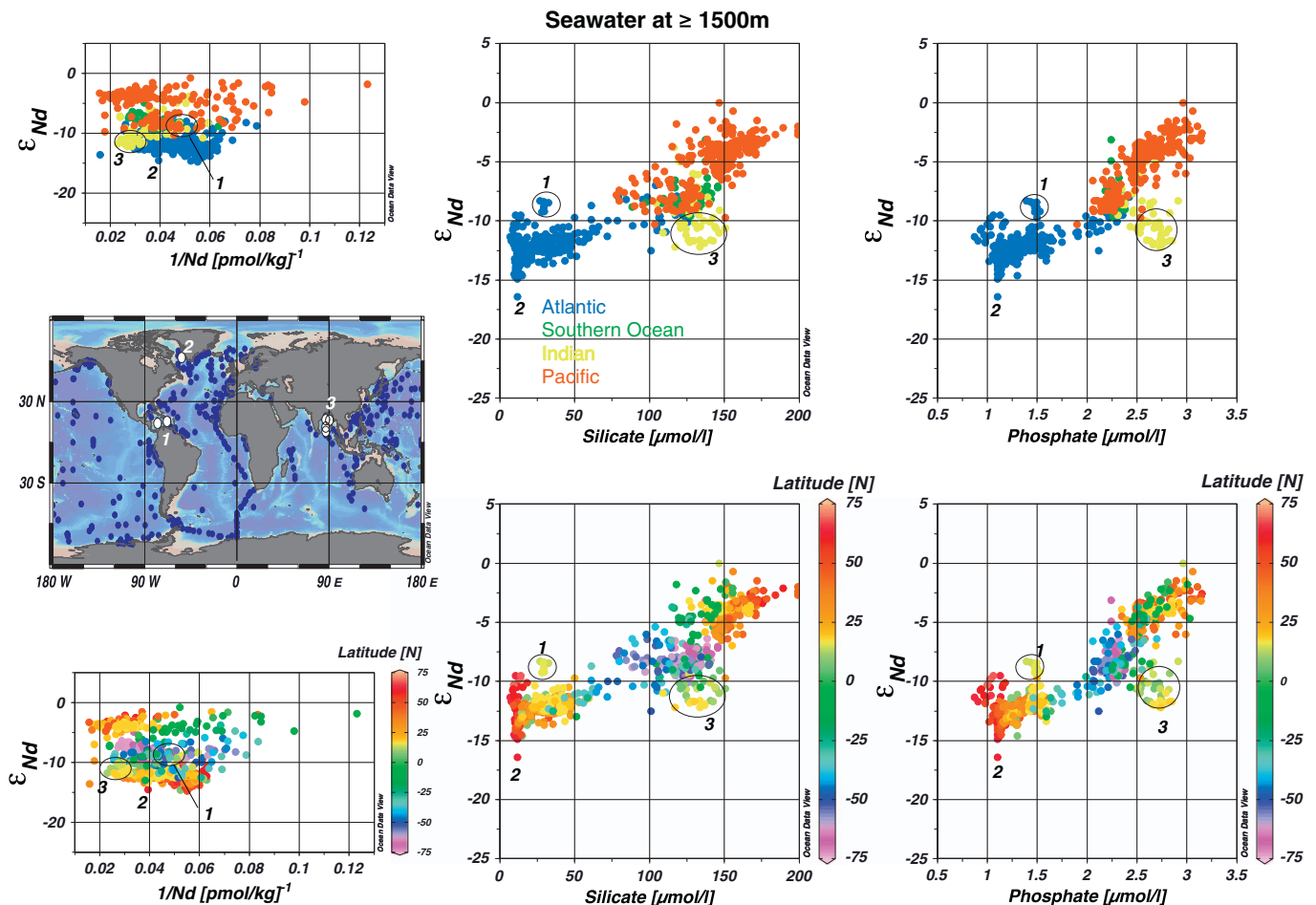
Fig. 3. Seawater multi-scatter plots for data at water depths deeper than 1500 m in the Atlantic, Southern Ocean, Indian and Pacific. All the data to create the plots are compiled in NEOSYMPA database. The numbers on the map show the area where seawater \epsilon_{Nd} values are offset from the general trend (see text for detail). The figures and the map are created using ODV (Schlitzer, 2015).
