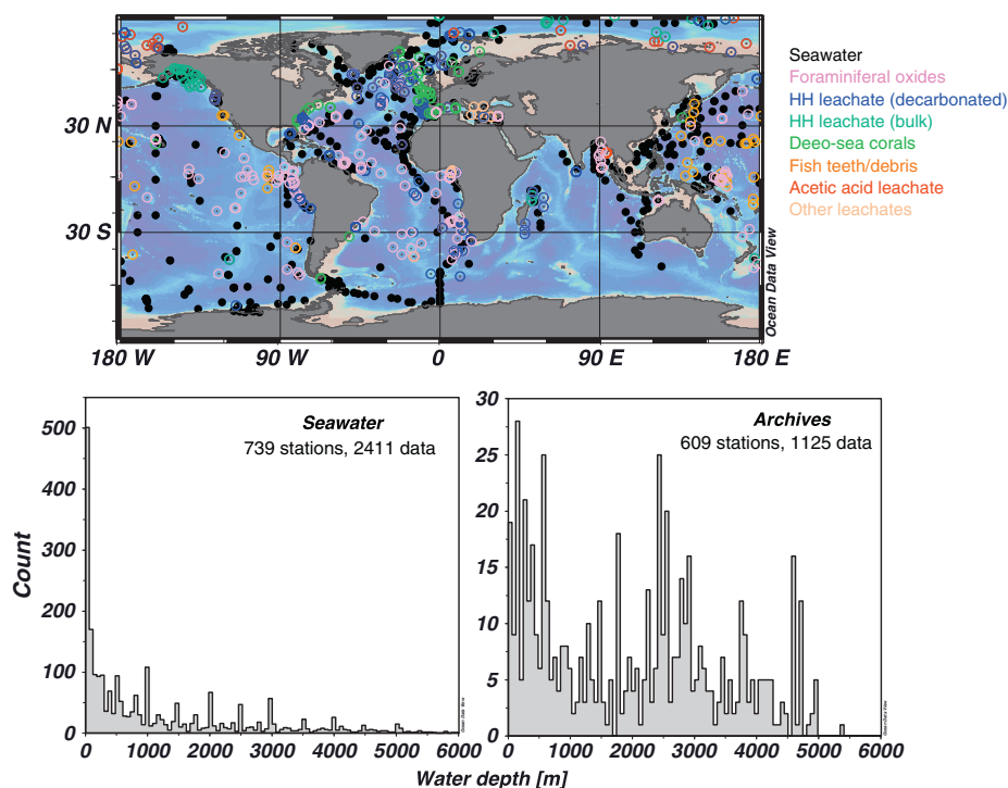
Fig. 1. Location map of all stations with \epsilon_{\text{Nd}} data together with vertical distribution of seawater and archives data stations. Black dots indicate seawater stations whereas open circles show various archive stations with color code. The map is visualized using the software Ocean Data View (ODV) (Schlitzer, 2015).
