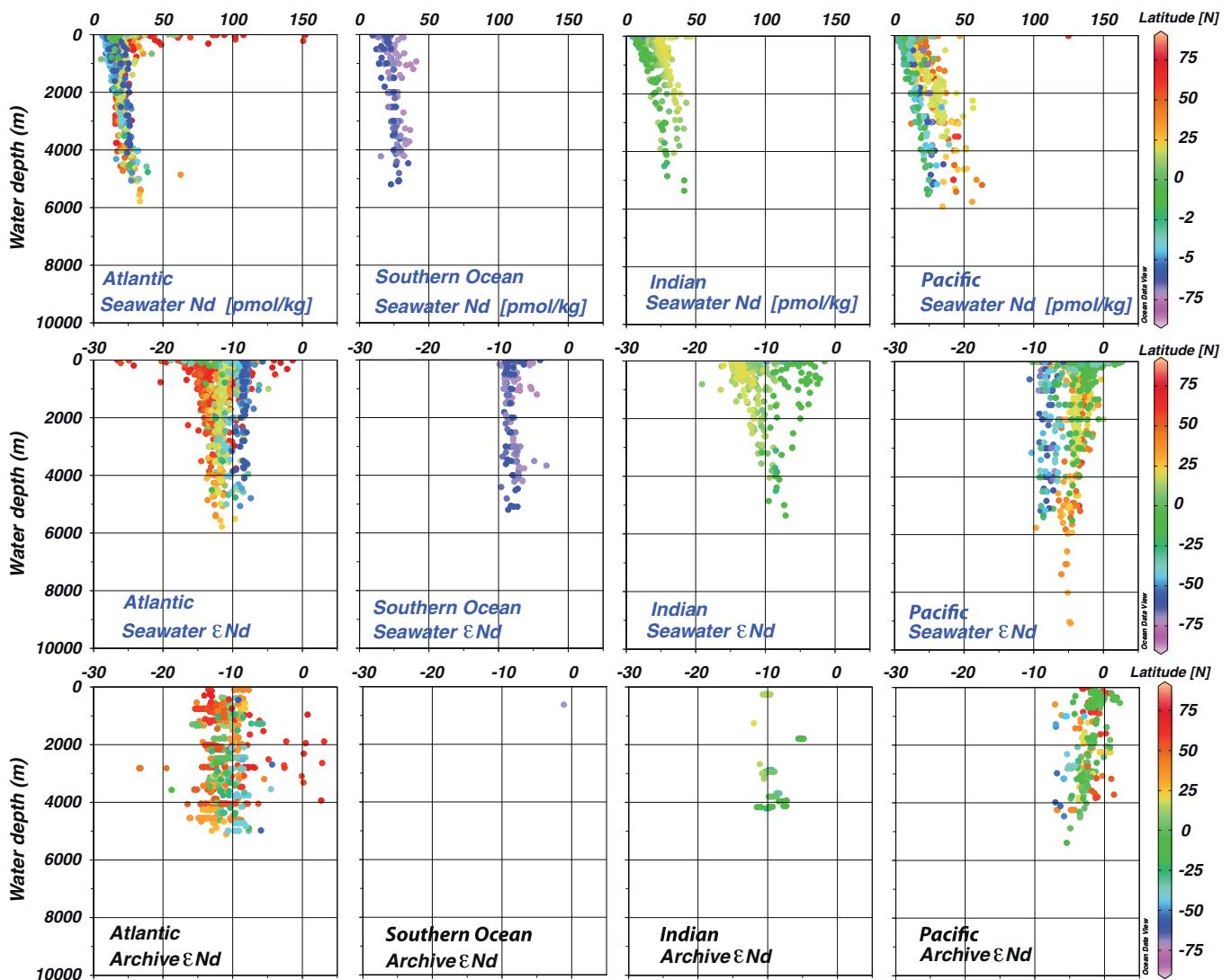
Fig. 2. Depth profiles of the compiled data in different oceanic basins. Seawater Nd concentrations (upper panels), seawater \epsilon_{Nd} values (middle panels), and archive \epsilon_{Nd} values (lower panels) for the Atlantic, Southern Ocean, Indian and Pacific. The color code indicates the latitudes of the data stations. The profiles are created using ODV (Schlitzer, 2015).
