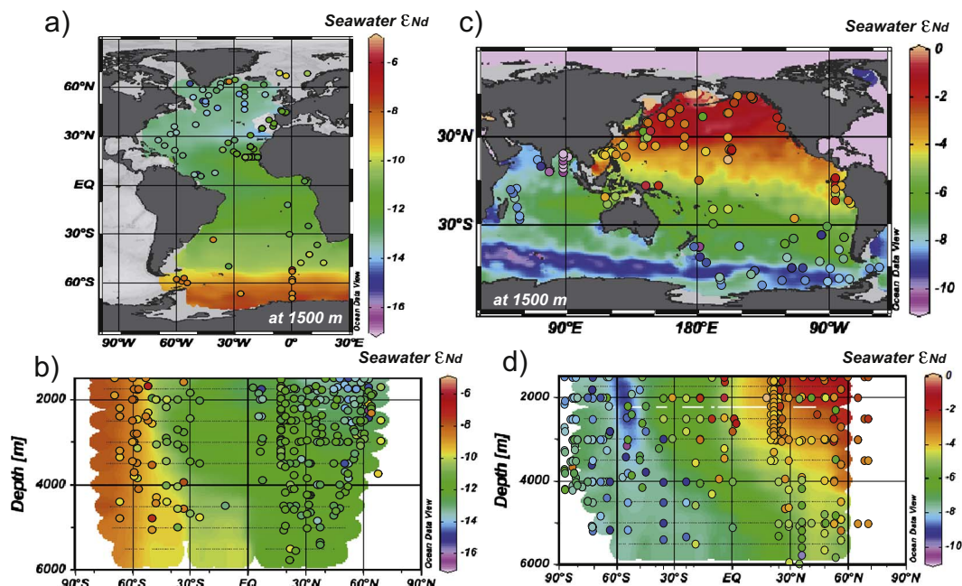
Fig. 7. Comparison between predicted deepwater \epsilon_{Nd} values (background color) with Eq. (1) (Atlantic at 50°S to 75°N) and Eq. (2) (global ocean except for the Atlantic at 50°S to 75°N) with observed seawater \epsilon_{Nd} values (color dots). The predicted deepwater \epsilon_{Nd} values at 1500 m are compared with observed seawater \epsilon_{Nd} values at \geq 1500 m in the Atlantic and Atlantic sector of the Southern Ocean (a) and the other oceanic regions (c). Zonally averaged latitudinal transect at 1500–6000 m of the Atlantic (b) and the Pacific (d). Note that the \epsilon_{Nd} scales are different with basins. The Atlantic sector of the Southern Ocean and the southernmost Atlantic (75°S to 50°S) is treated as a buffer zone where deepwater \epsilon_{Nd} values are calculated by both Eqs. (1) and (2), and weighted-averaged values considering latitudinal position are shown. All the figures and maps are created using ODV (Schlitzer, 2015).
