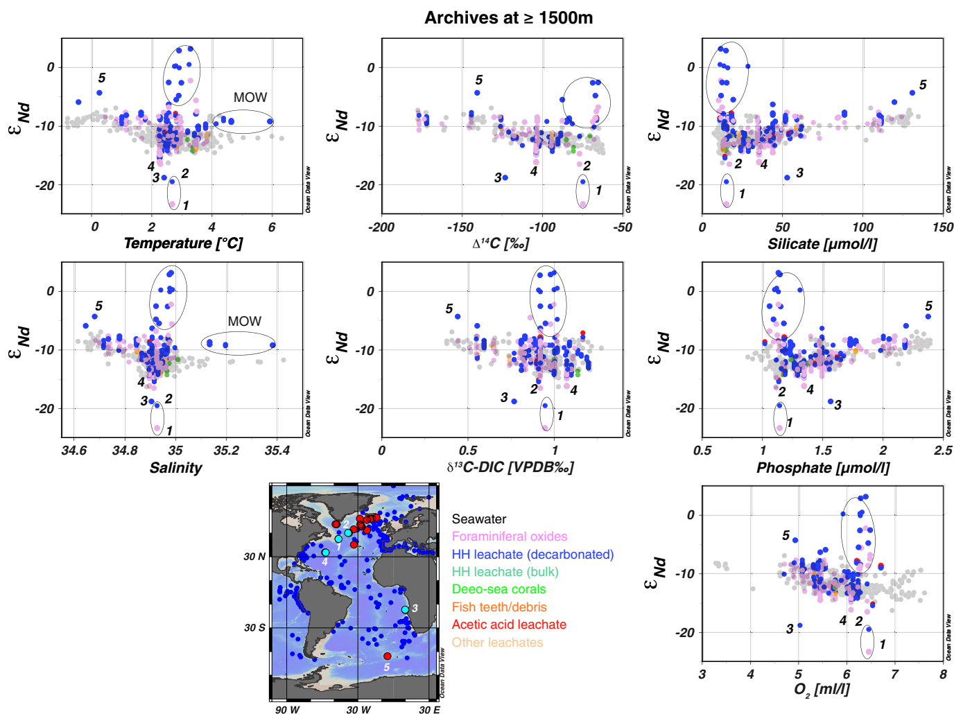
Fig. 5. Basin-scale archive multi-scatter plots at \geq 1500 m. a) Atlantic, b) Indian, and c) Pacific and Pacific sector of the Southern Ocean. The red and blue stations on the maps indicate the sites with positive and negative offsets, respectively. The color code shows different archive types and gray dots indicate seawater values shown in Fig. 4abc. There is no archive data from deepwater depths ( \geq 1500 m) in the Atlantic and Indian sectors of the Southern Ocean. The numbers on the map show the area where seawater \epsilon_{Nd} values are offset from the general trend (see text for detail). The figures and the maps are created using ODV (Schlitzer, 2015).
