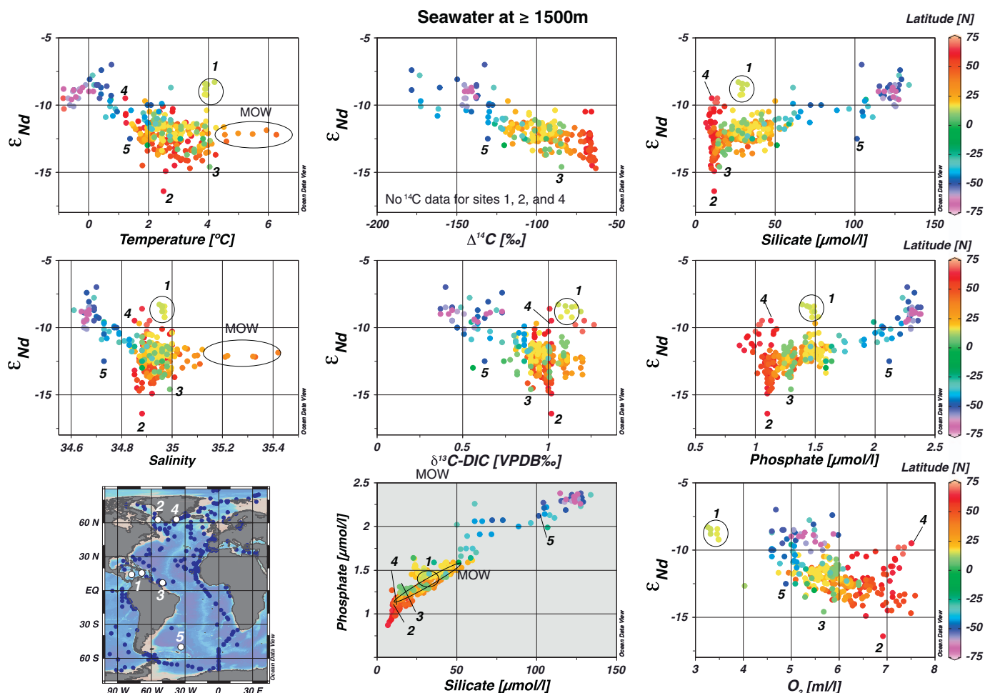
Fig. 4. Seawater property-property plots for water depths deeper than 1500 m. The color code shows latitudes (a and c) or longitude (b) of data stations. a) Atlantic and Atlantic sector of the Southern Ocean, b) Indian, and c) Pacific and Pacific sector of the Southern Ocean. MOW = Mediterranean Outflow Water. The numbers on the maps show the sites where seawater \epsilon_{Nd} values are offset from the general trend (see text for detail). The figures and the maps are created using ODV (Schlitzer, 2015).
