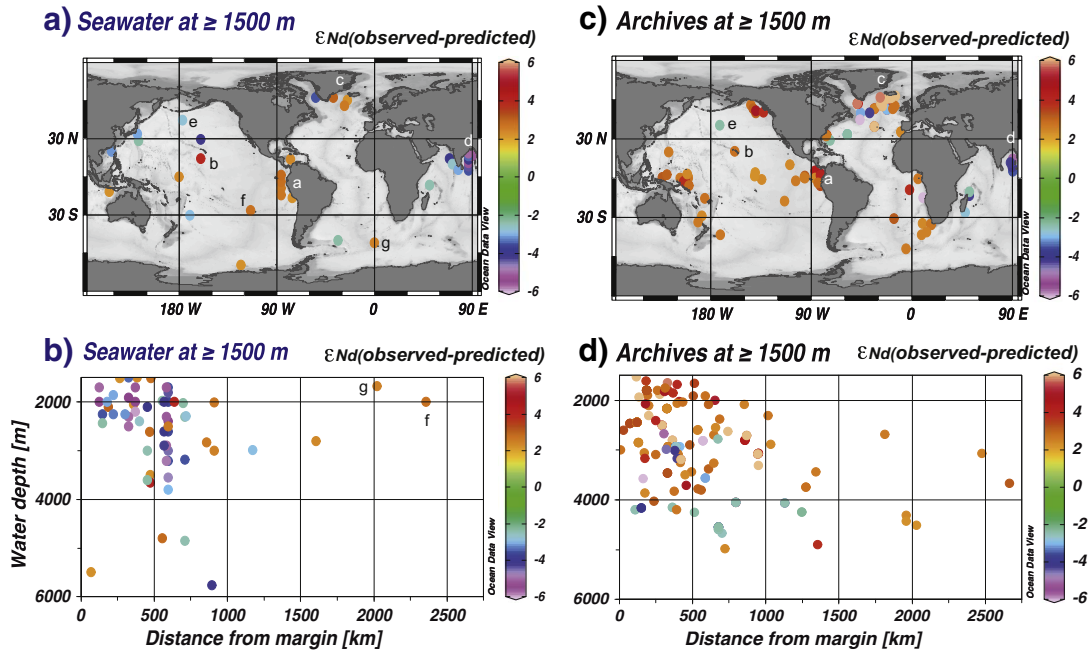
Fig. 9. Distribution of sites where the seawater and archive \epsilon_{Nd} values are significantly affected by local/regional detrital inputs. Maps showing the sites at \geq 1500 m for seawater data (a) and archive data (c). Relationship between the distance from margin and water depth for seawater data (b) and archive data (d). Labels “a” to “g” show sites discussed in the text. All the figures and maps are created using ODV (Schlitzer, 2015).
