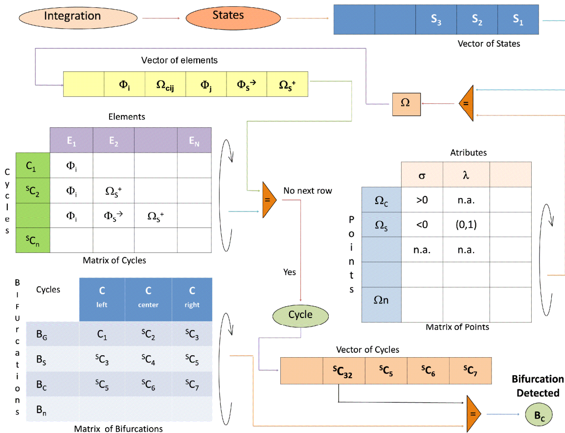
Figure 3. General method of comparison of sequences of cycles and bifurcations.
