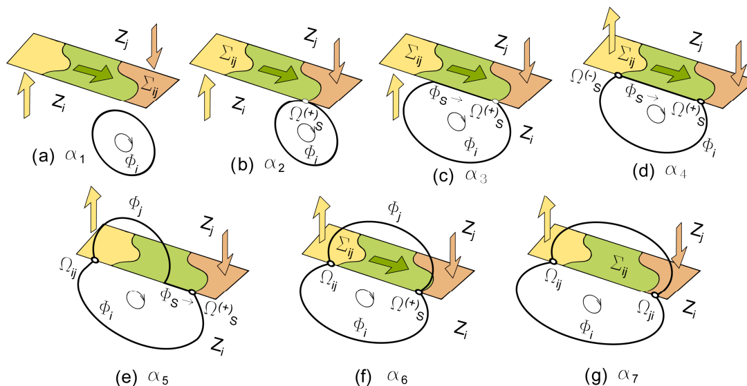
Figure 1. Grazing (a)-(c), Switching (c)-(e) and Crossing (e)-(g) bifurcations.
