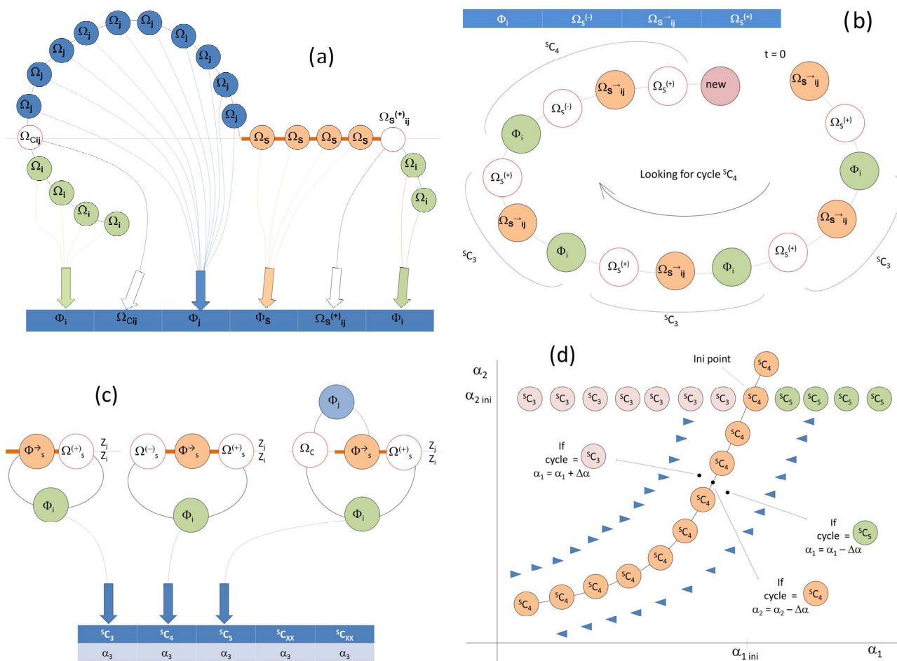
Figure 2. Implementation of Cycle Bifurcation. (a) Process of filling the vector with elements appearing in the numeric integration; (b) Searching process for a specific cycle; (c) Cycle tracking process for bifurcations detection; (d) Cycle continuation process.
