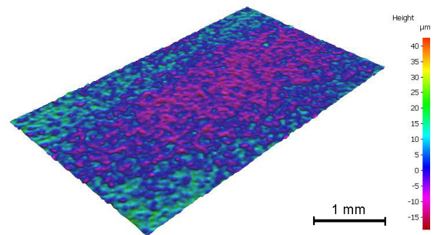
FIGURE 5. Colour filtered image of the surface of sample 23, 2.5 × magnified (voltage 70 V, T_{on} = 10 \mu s , T_{off} = 30 \mu s , wire feed 14 m/min, current 25 A).
