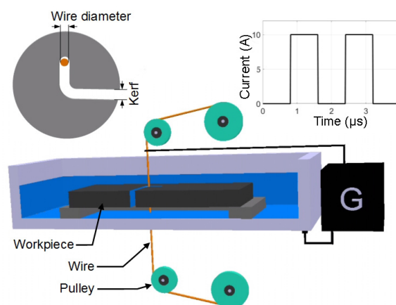
FIGURE 1. Diagram of wire electrical discharge machining process.
