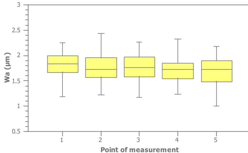
FIGURE 11. Values W_a in individual points of measurement on all samples made of titanium alloy Ti-6Al-4V with heat treatment.
