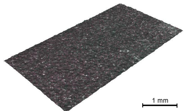
FIGURE 8. Non-filtered image of the surface of sample 30, 2.5 \times magnified (voltage 70 V, T_{on} = 6 \mu\text{s} , T_{off} = 30 \mu\text{s} , wire feed 14 m/min, current 35 A).
