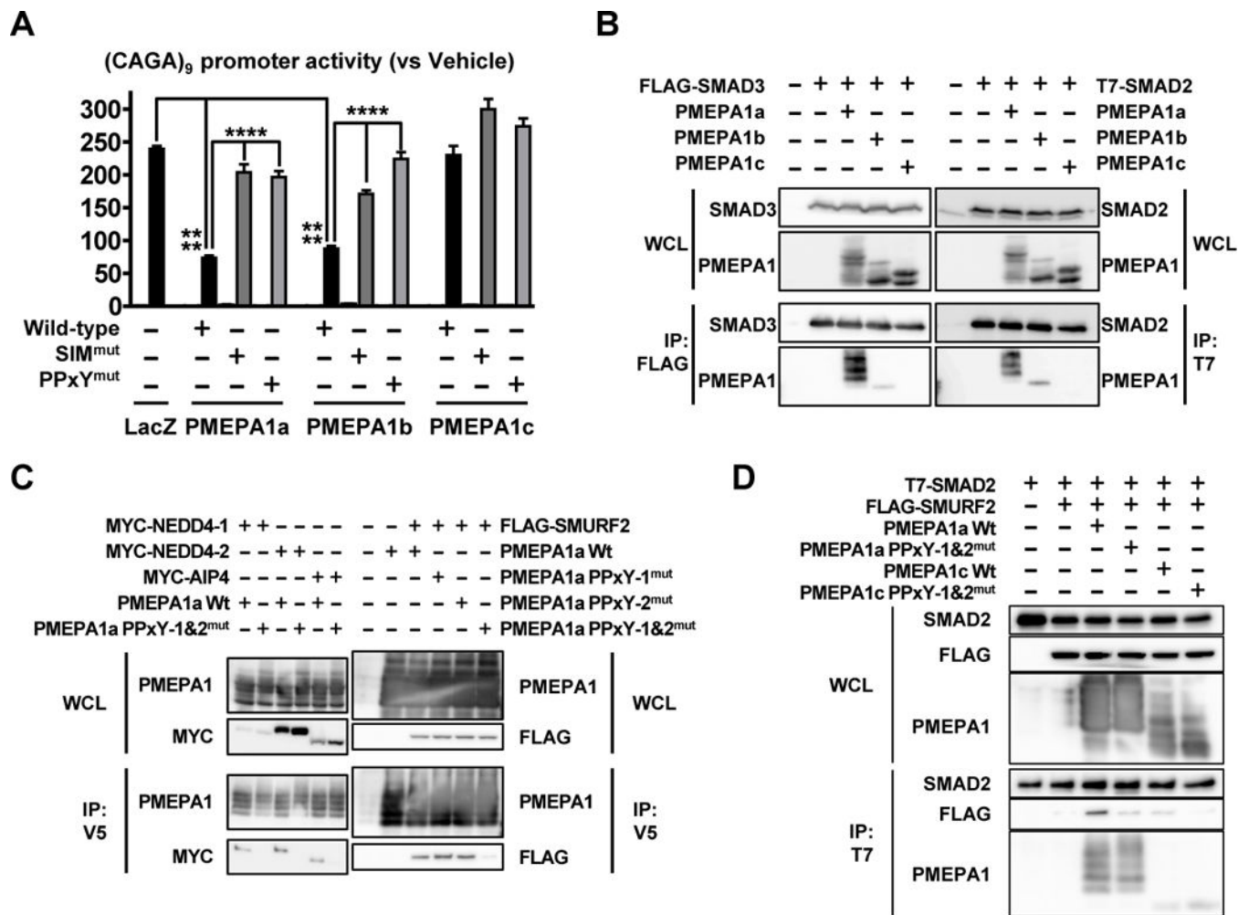
Figure 5. Only membrane-bound PMEPA1 inhibits TGFβ signaling pathway by interacting with SMAD2/3 and HECT E3 ubiquitin ligases
