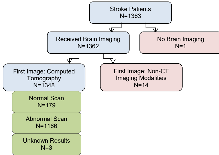
Figure 1: Cohort Schematic (N=1363)
