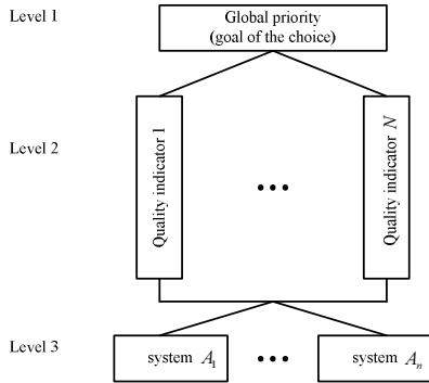
Fig. 1. Decomposition of the problem of choice in the levels hierarchy
