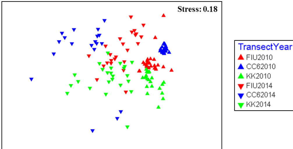
Figure 10. Temporal variability within three sites (Red=FIU, Blue=CC6, and Green=KK) across a four year time-span (▲ 2010/▼ 2014) based on Nonmetric Multidimensional Scaling (nMDS) analysis using Bray-Curtis similarity coefficient.
