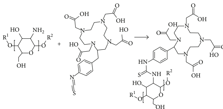
FIGURE 1: CHS-p-SCN-Bn-DOTA reaction.
