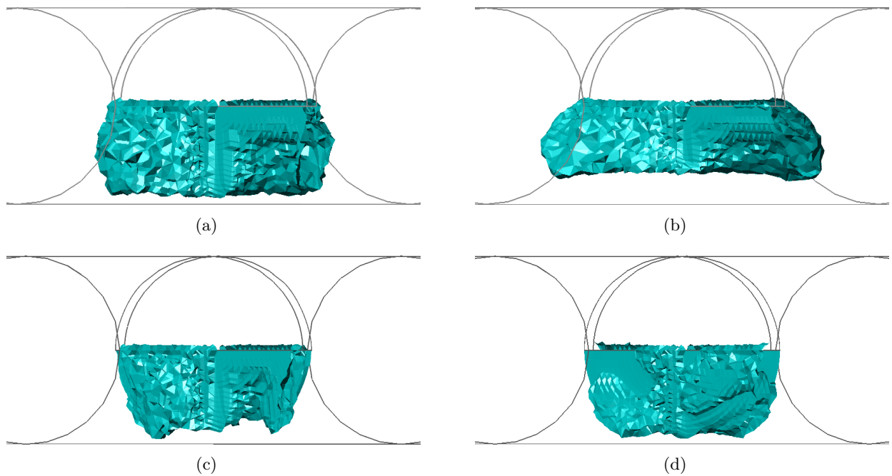
Figure 23: Side view of the crack pattern from (a) Rankine Isotropic Damage, (b) Rankine Plasticity, (c) Drucker-Prager isotropic damage and (d) Drucker-Prager plasticity solutions.
