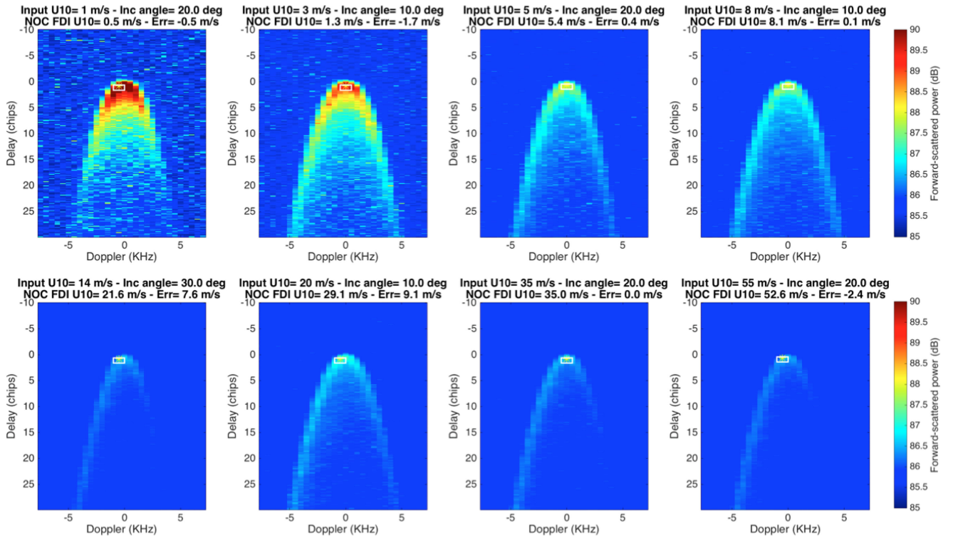
Fig. 20. Examples of L1 DDM produced by the GEROS-SIM M2 module with the TDS-1 configuration. The L1 DDM correspond to different wind speeds and incidence angles as indicated in the legend of each subplot (Inc: 0.1^\circ corresponds to nadir).
