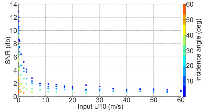
Fig. 21. Signal-to-noise ratio obtained with the GEROS-SIM M5 scatterometry module applied to M2 L1 DDM obtained for different input wind speed and incidence angle of the specular point (Inc: 0.1^\circ corresponds to nadir).
