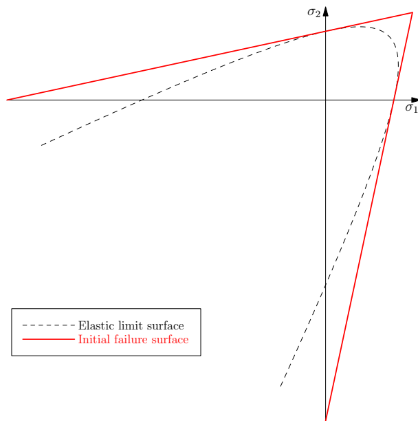
(c) Elastic limit surface of hyperbolic type
