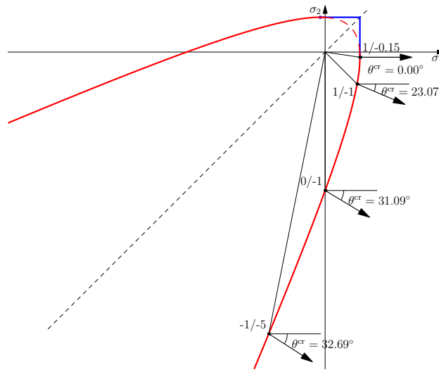
(c) Hyperbolic type ( \rho = 4.0 )
