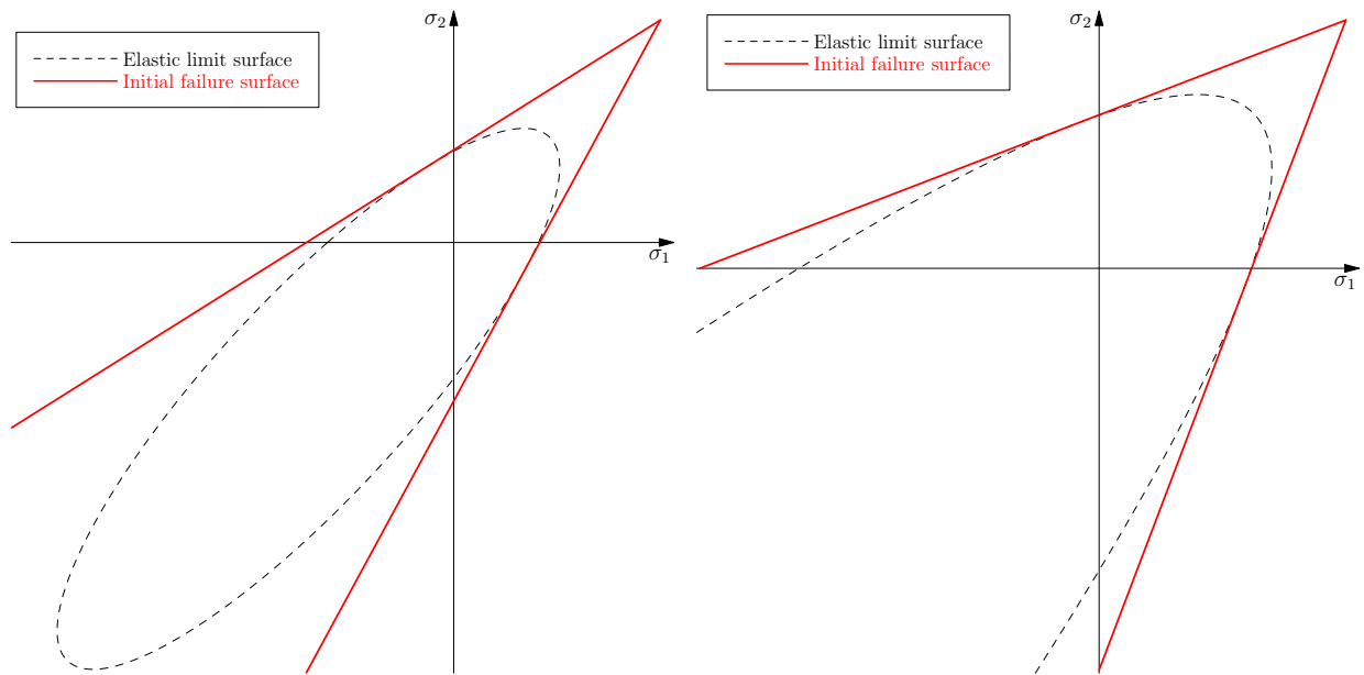
(a) Elastic limit surface of elliptic type
