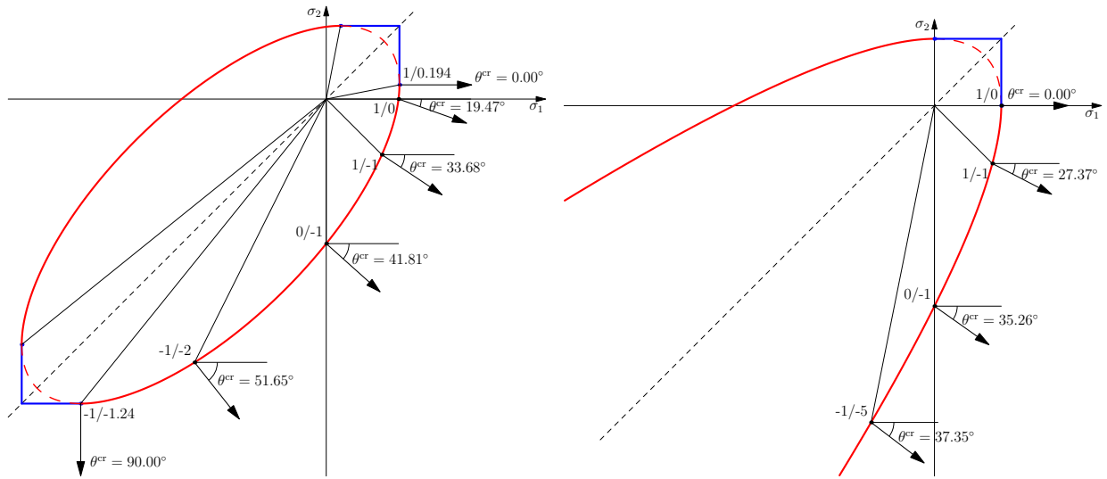
(a) Elliptic type ( \rho = 2.0 )
