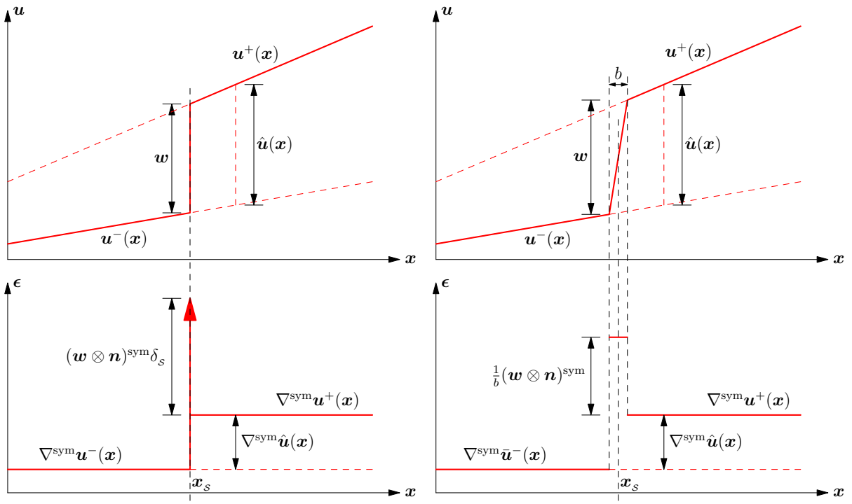
(a) Displacement/strain fields around a strong discontinuity
