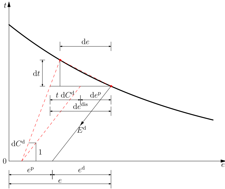
Figure 7: 1-D definition of the dissipative deformation vector rate and its damage/plastic components
