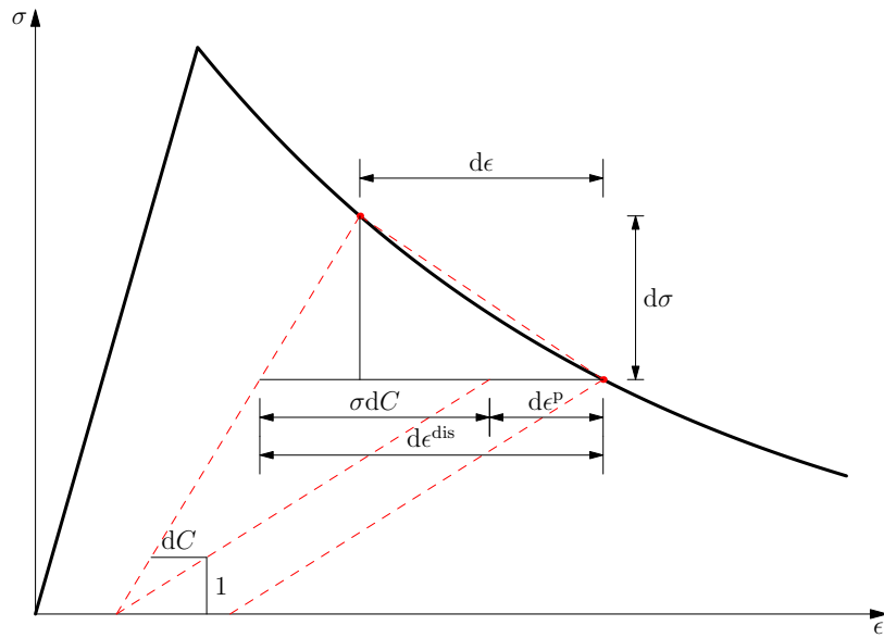
Figure 1: 1-D definition of the dissipative strain rate tensor and its damage/plastic components
