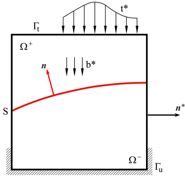
Figure 3: Problem setting in an elastic solid medium with an internal discontinuity
