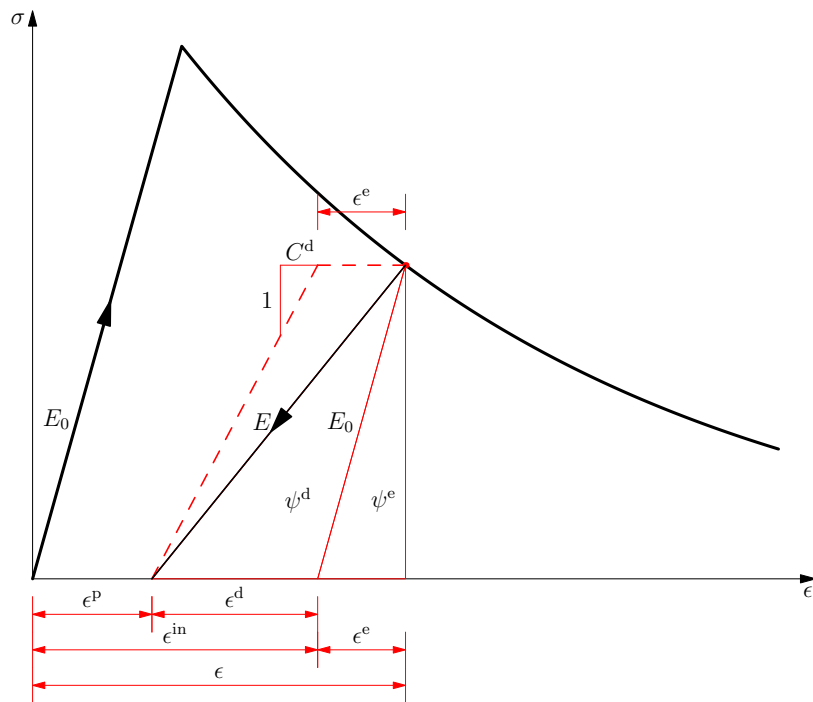
Figure 2: Different kinematic decompositions adopted in the unified elastoplastic damage model
