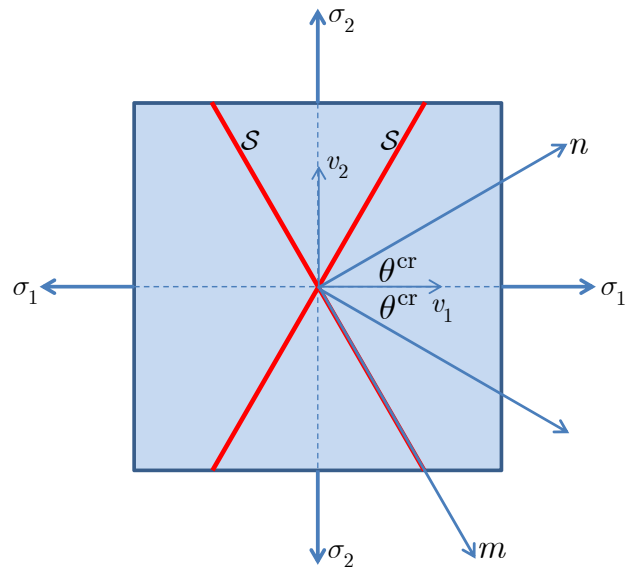
Figure 8: Definition of the discontinuity angle
