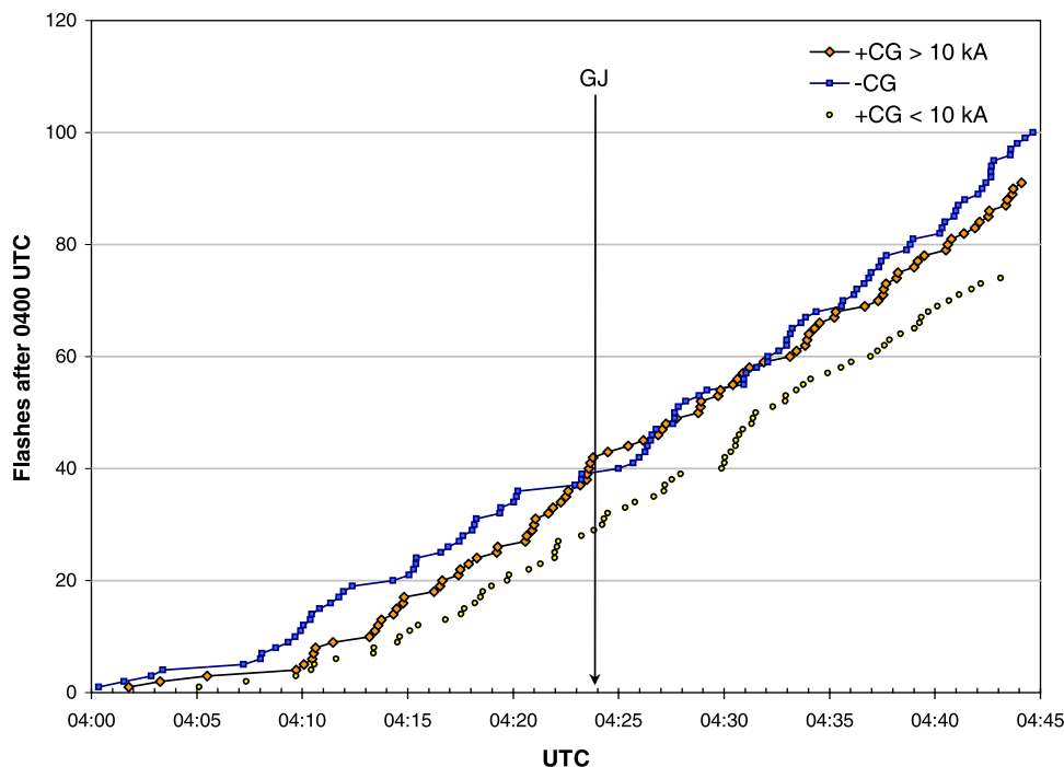
Figure 7. Cumulative flash rates (by NLDN) for the portion of the far storm near the direction of the gigantic jet, indicated by a box in Figure 4. A rapid rise of +CG flash rates occurs before the gigantic jet, during a 5-min period of almost absent –CG flashes, followed by a relative pause in +CG rates. NLDN +CG flashes <10 kA are considered a subset of intracloud flashes.
