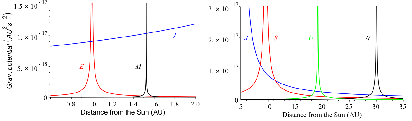
Figure 2. Values of the gravity potential (in \text{au}^2 \text{s}^{-2} ) of the Earth (E), Mars (M) and Jupiter (J) in the heliocentric region including the orbits of the Earth and Mars (left), and gravity potential of Jupiter (J), Saturn (S), Uranus (U) and Neptune (N) in the heliocentric region corresponding to the outer Solar system.
