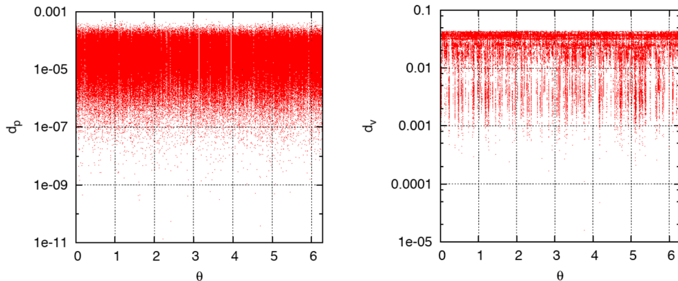
Figure 13. Minimum distances d_p (positions, left) and d_v (velocities, right) between points of the invariant manifolds at the section \Sigma_{R_1} of the Uranus and Neptune bicircular problems. See the text for more details.
