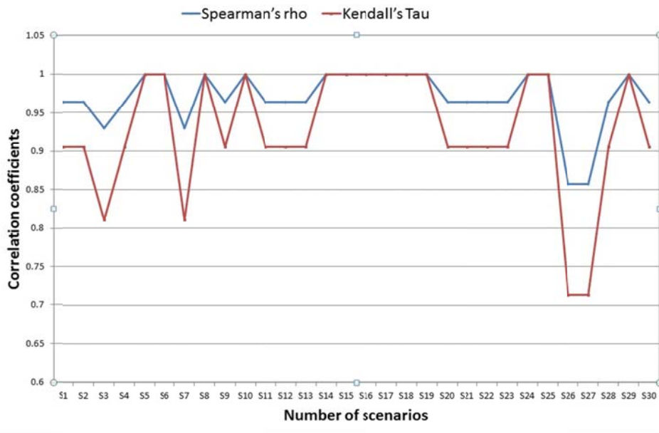
Fig. 1: Spearman's rho and Kendall's tau correlation coefficients
