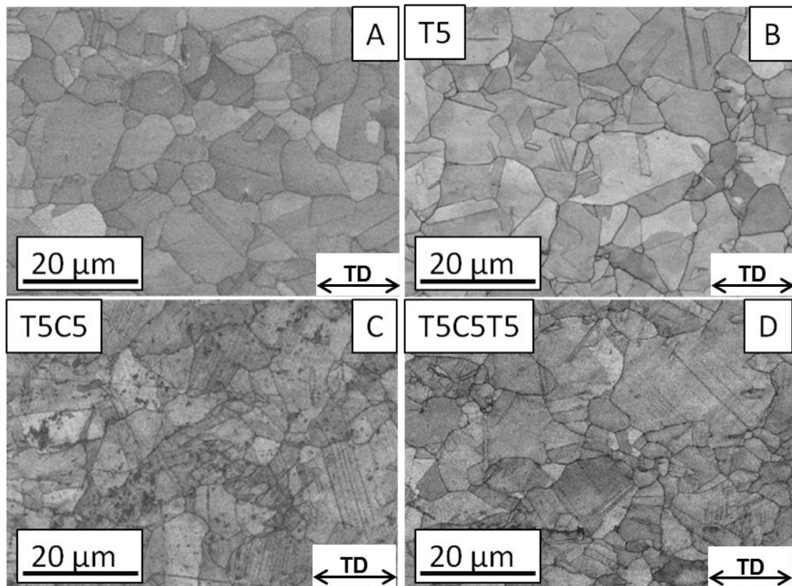
Fig.7. Evolution of the microstructure of Fe-17Mn-0.7C-2Al TWIP steel during the cyclic test at 5% pre-strain. Image Quality maps obtained by EBSD with a step size of 0.1 \mu\text{m} . A) Initial material; B) First tensile stage at 5% strain (T5); C) Compressive stage at -5% strain (T5C5); D) Second tensile stage at 5% strain (T5C5T5). TD: Tensile direction.
