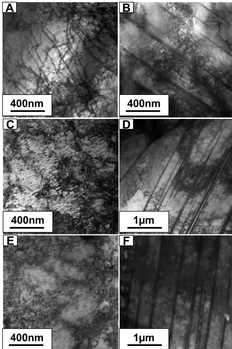
Fig.8. TEM micrographs showing the evolution of dislocation structure and mechanical twins for the cyclic test at 5% pre-strain. A and B) After first tensile stage at 5% strain (T5); C and D) After compressive stage at -5% strain (T5C5); E and F) After the second tensile stage at 5% strain.
