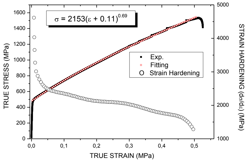
Fig.3. Tensile stress-strain curve for the Fe-17Mn-0.7C-2Al TWIP steel together with the fitting curve using Swift's hardening law. The strain hardening evolution with strain is also displayed.
