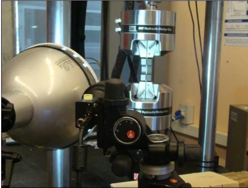
Fig. 2. Assembly of the anti-buckling device and the video-extensometer for the cyclic test of sheet samples.
