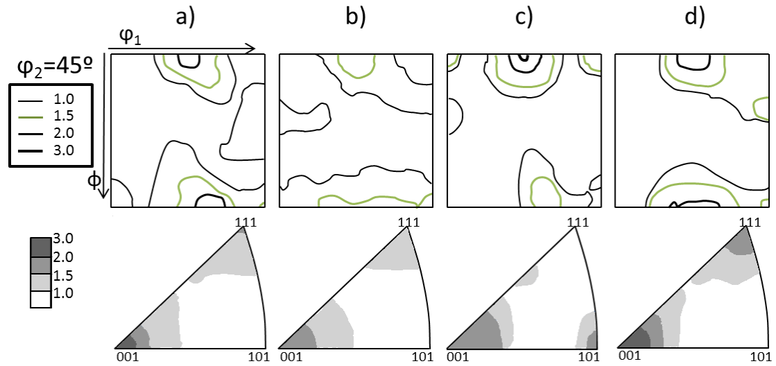
Fig.9. ODF in \phi_2 = 45^\circ sections and IPF for the as-received material and after different strain levels. a) as-received material; b) after 5% tensile strain (T5) c) after compressive stage to -5% strain (T5C5) and d) after second tensile stage at 5% strain (T5C5T5).
