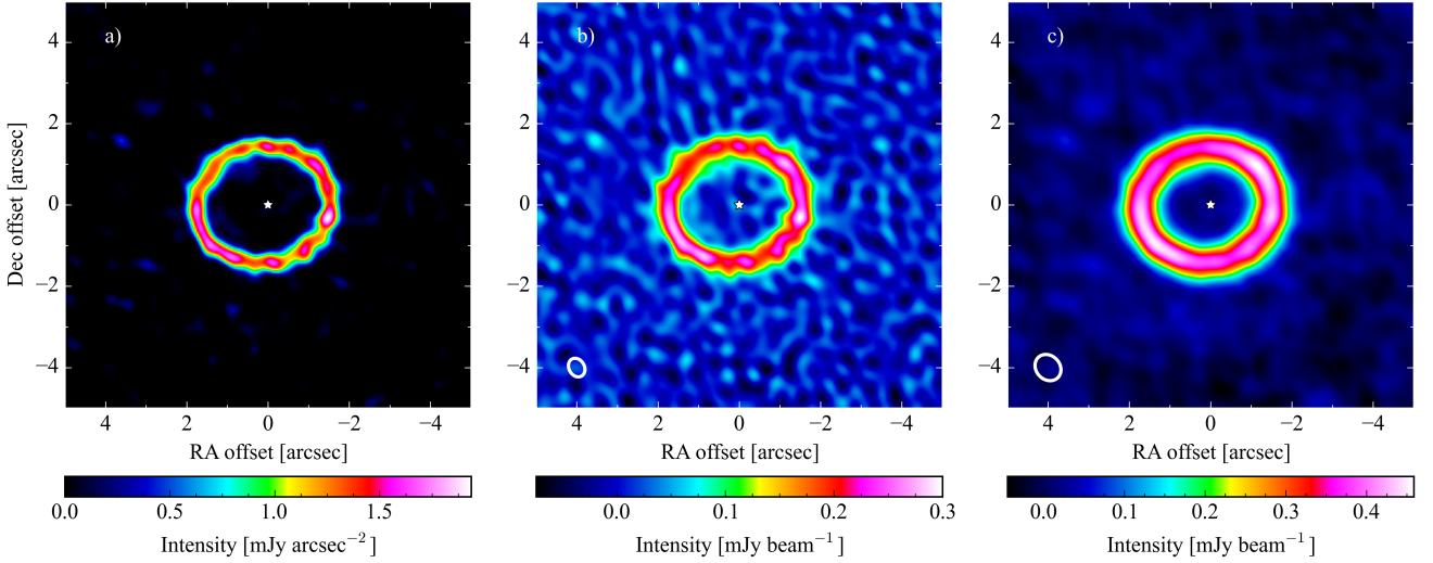
Figure 1. ALMA dust continuum maps at 220 GHz (Band 6). a) MEM non-parametric model (regularized with the maximum entropy method). b) Restored image adding residuals and convolving with a synthetic beam corresponding to Briggs weighting ( 0''.47 \times 0''.36 ). c) Restored image adding residuals and convolving with a synthetic beam corresponding to natural weighting ( 0''.69 \times 0''.58 ). The respective beams are represented by white ellipses. The x- and y-axes indicate the offset from the stellar position in R.A. and decl. in arcsec, i.e. north is up and east is left. The stellar position is marked with a white star.
