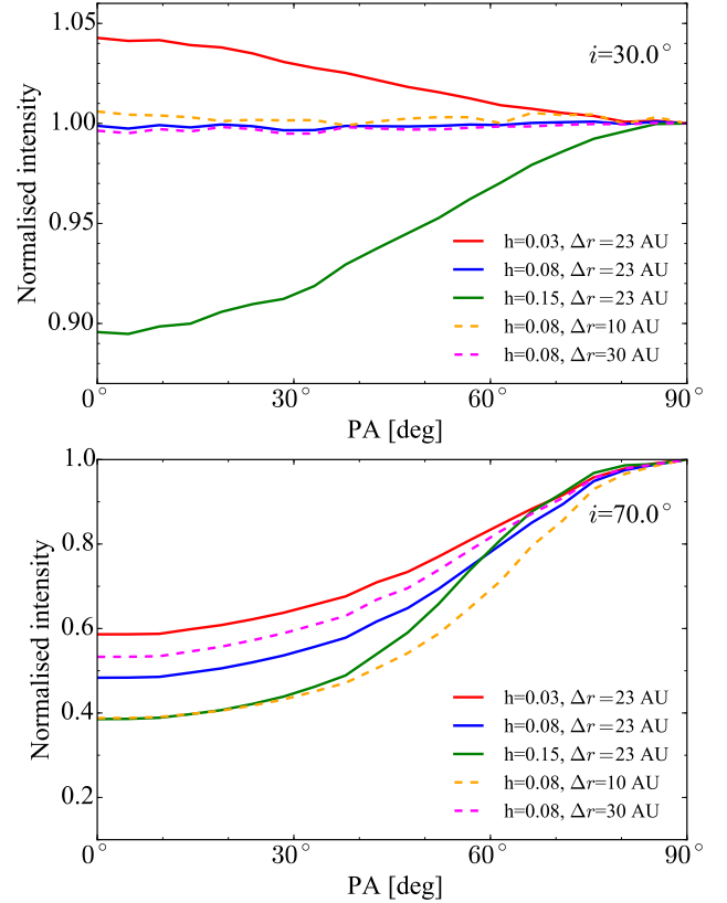
Figure 10. Intensity profiles along the ring projected ellipse on sky obtained from simulated Clean images without noise and using our best fit ring model. The values are normalised to the intensity at the ring semi-major axis (PA=90°). The upper panel corresponds to a disc inclined by 30°, while the lower to 70°. In red, blue and green lines we present three different profiles for disc aspect ratios of 0.03, 0.08 and 0.15 with \Delta r fixed to 23 AU, while in dashed lines we present profiles varying h and \Delta r .
