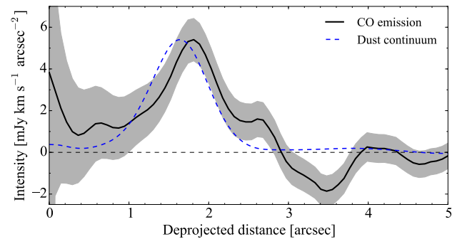
Figure 4. Mean intensity at all azimuths (black line) integrating from -2.8 km s ^{-1} and 2.0 km s ^{-1} with respect to 230.538 GHz, in the Barycentric reference frame. The profile is extracted from the dirty map with natural weights of the continuum subtracted visibilities. The grey area represents the 68% confidence region. In blue we also present the mean intensity of the dust continuum presented in Fig. 2 in an arbitrary scale.
