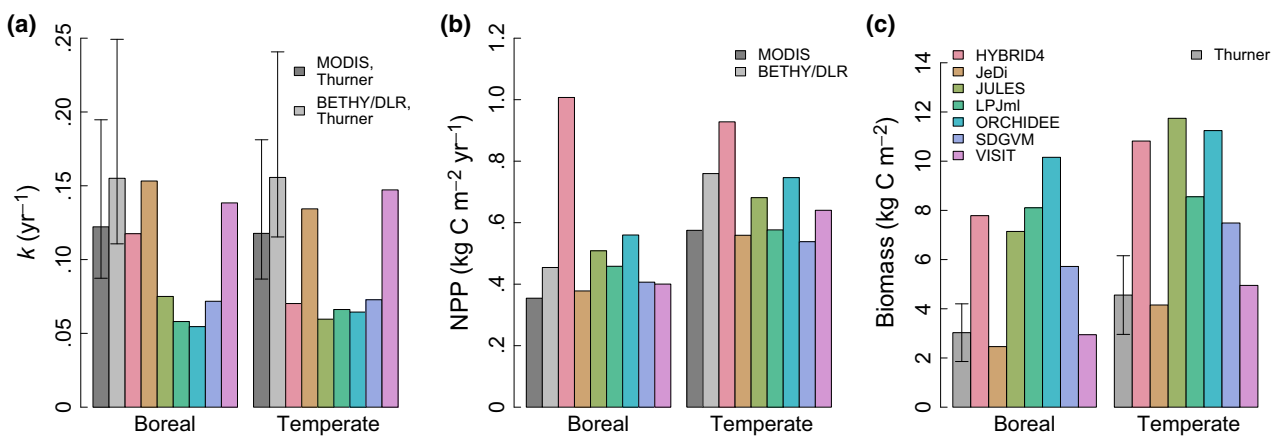
FIGURE 2 Comparison of observation-based and simulated (a) mean k , (b) mean NPP, and (c) mean biomass in boreal and temperate forests (cf. Appendix S5). All forest areas at .5^\circ resolution are included, but accounting for nonforest vegetation within these areas. Simulated k , NPP, and biomass are obtained from GVMs participating in ISI-MIP (HYBRID4, JeDi, JULES, LPJml, ORCHIDEE, SDGVM, VISIT). In (a), the harmonic mean of k has been calculated. Observation-based k has been derived based on both available NPP products (MODIS and BETHY/DLR), using the biomass product from Thurner et al. (2014). Uncertainty bounds in observation-based k represent the uncertainty in the biomass product. In (b), observation-based NPP is available from two products (MODIS and BETHY/DLR). No comparable uncertainty estimates are available for NPP. In (c), observation-based biomass is obtained from Thurner et al. (2014), including an uncertainty estimate
