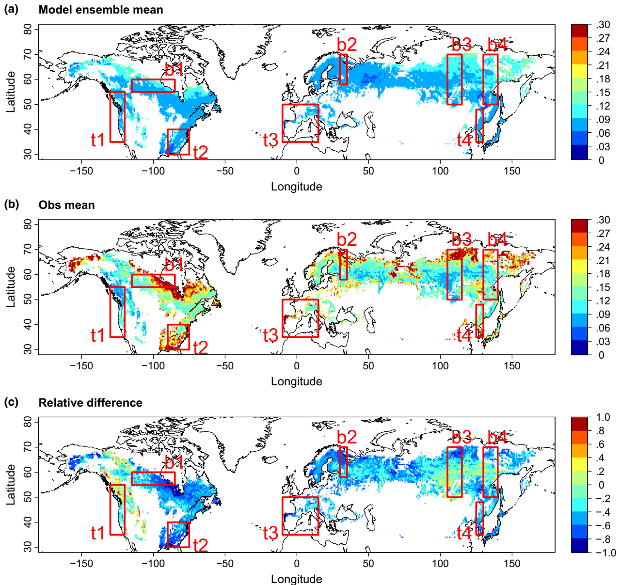
FIGURE 1 Spatial patterns of forest k [ \text{yr}^{-1} ] as the ratio of NPP to biomass (a) simulated by GVMs participating in ISI-MIP (ensemble mean of HYBRID4, JeDi, JULES, LPJml, ORCHIDEE, SDGVM, and VISIT) and (b) based on satellite data (Obs mean; using an average of MODIS and BETHY/DLR NPP products and observation-based biomass from Thurner et al. 2014). The relative difference of (a) with respect to (b) is shown in (c). Only areas with at least 40% forest cover are considered. Red boxes show selected transects (see Appendix S1): b1 Canada, b2 Karelia/Western Russia, b3 Central Siberia/Baikal, b4 Eastern Siberia, t1 Western North America, t2 South-Eastern North America, t3 South-Western Europe, t4 North-Eastern China/Korea
