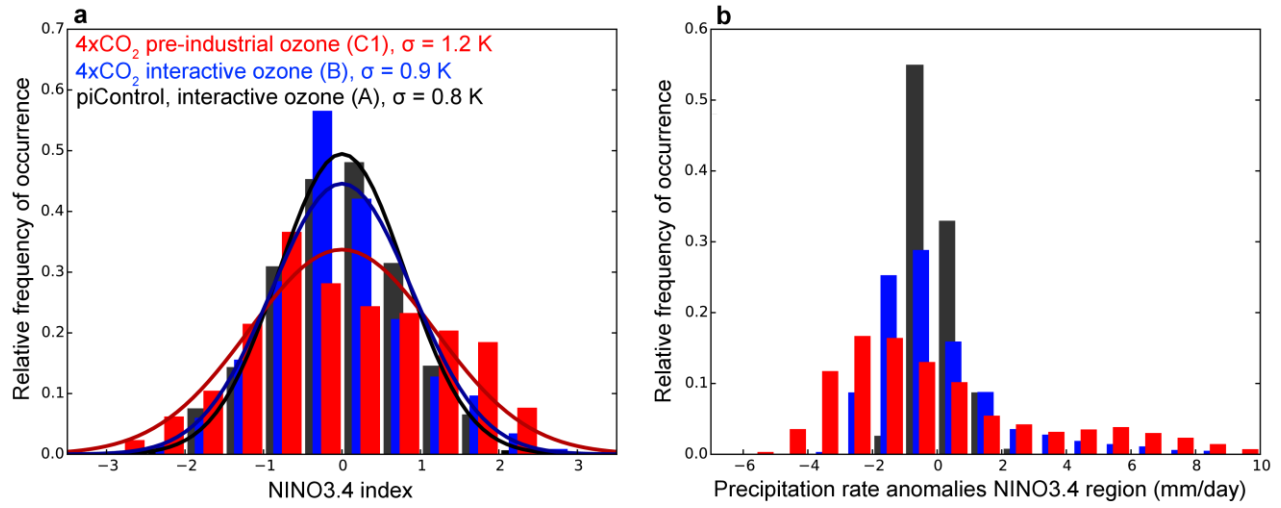
Figure 1. Normalized histograms of NINO3.4 (a) temperature and (b) precipitation rate anomalies as relative frequencies of occurrence, color coding for the integrations as in (a).
