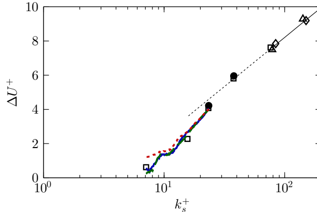
Figure 13: Hama roughness function for the temporal sweep with modelled roughness at fixed k = h/40 , where k_s^+ \approx 1.6k^+ . Symbols: black symbols, steady flow data for the same modelled roughness (Chung et al. 2015); —, sweep data for \Delta_{p, Re_\tau=180} = 0.03 (slowest sweep); - - -, sweep data for \Delta_{p, Re_\tau=180} = 0.07 ; - · - ·, sweep data for \Delta_{p, Re_\tau=180} = 0.15 (fastest sweep).
