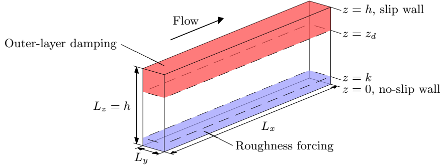
Figure 1: Half-height minimal-span channel, showing the roughness forcing zone (2.2) and the outer-layer damping zone (2.3). No-slip wall at z = 0 and free-slip wall at z = h .
