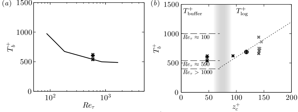
Figure 14: (a) Buffer-layer bursting period T_b^+ against friction Reynolds number. Solid line denotes data of Jiménez et al. (2005), symbols are current data for buffer-layer minimal channels. (b) Bursting period T_b^+ against wall-normal critical height z_c^+ . Symbols: \times , Re_\tau = 590 standard-height channel; \dagger , Re_\tau = 590 half-height channel; \oplus , Re_\tau = 2000 half-height channel. Lighter grey symbols denote shorter streamwise channel lengths. Line styles: —, buffer-layer bursting period at different Re_\tau ; - - -, log-layer bursting period T_b U_\tau / z_c = 6 (Flores & Jiménez 2010; Hwang & Bengana 2016).
