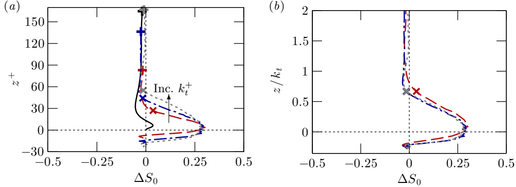
Figure 19: Difference \Delta S_0 between sweep and ejection stress contributions (Raupach 1981) as a function of (a) z^+ and (b) z/k_t . Line styles: —, smooth wall (sm.396); - - -, k_t^+ \approx 40 (40.198); - · - ·, k_t^+ \approx 63 ; - - -, k_t^+ \approx 80 . Symbols: +, z_c^+ ; ×, pyramid crest.
