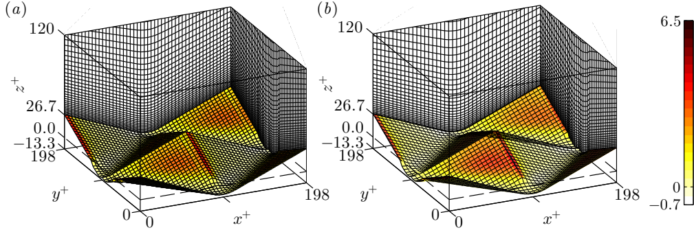
Figure 17: Pyramid geometry and body-fitted mesh for pyramid with k_t^+ = 40 , \lambda^+ = 198 at Re_\tau = 840 for (a) normal mesh 40_198 and (b) finer mesh 40_198.f. Only every (a) fifth or (b) tenth wall-normal node is shown, and only every second spanwise and streamwise node in (b). Contour shows time-averaged total drag (viscous + pressure) force per unit area.
