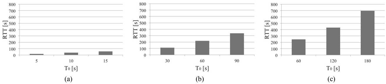
Fig.7. Round Trip Time varying the Data Rate: (a) 1 packet every 5 seconds, (b) 1 packet every 30 seconds, (c) 1 packet every 60 seconds.
