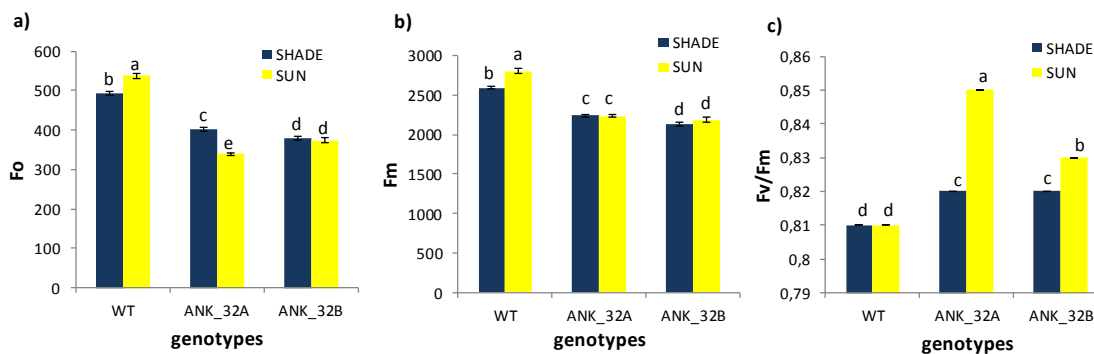
Figure 1. Selected parameters derived from fast fluorescence kinetic measurements in the sun and the shade wheat. a) minimum fluorescence from dark-adapted leaf - F_0 , b) maximum fluorescence from dark - F_m , c) related to maximum photochemical efficiency of PSII - F_v/F_m . Letters indicate significant differences at P < 0,05 according to Duncan's multiple range tests.
